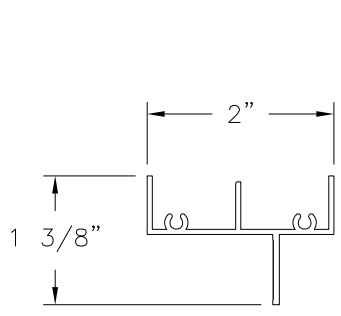
MAIN FRAME FINLESS INSTALLATION ALUMINUM 6063-T5 (CM-18524)
