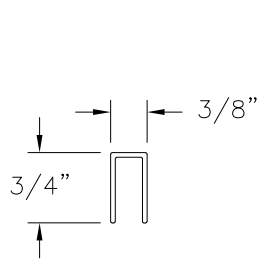
GLAZING BEAD INSULATED GLASS ALUMINUM 6063-T5 (CM-18540)
