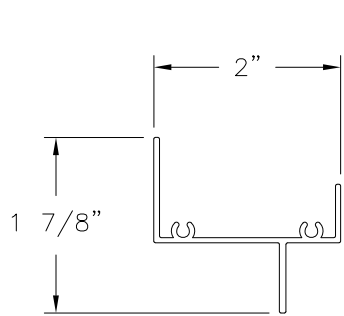
MAIN FRAME FINLESS INSTALLATION WITH FLANGE ALUMINUM 6063-T5 (CM-18524)
