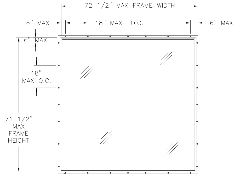
SERIES 185 ALUMINUM FIXED WINDOW EXTERIOR VIEW
