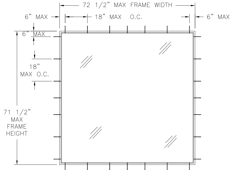
SERIES 185 ALUMINUM FIXED WINDOW EXTERIOR VIEW
