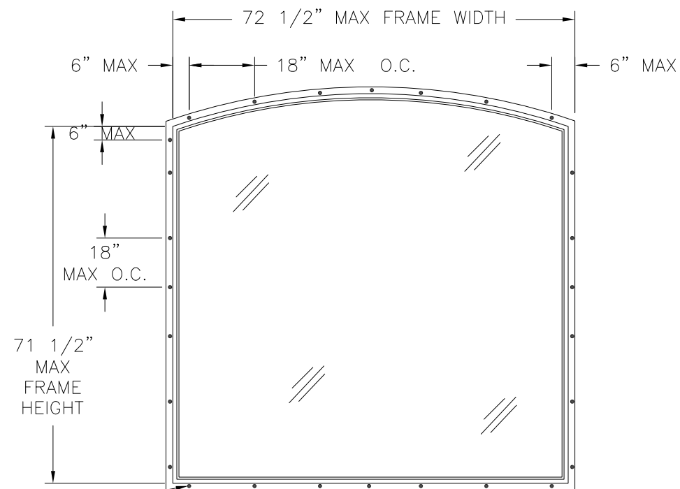
SERIES 185 ALUMINUM FIXED DESIGNER WINDOW EXTERIOR VIEW
