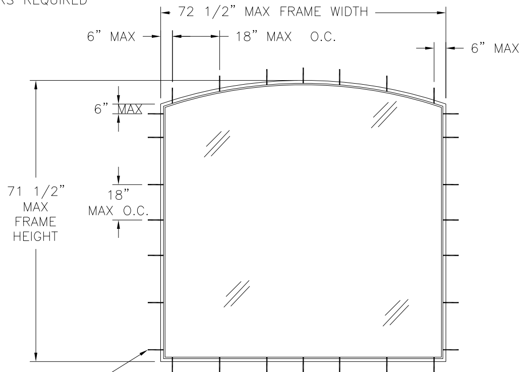
SERIES 185 ALUMINUM FIXED DESIGNER WINDOW EXTERIOR VIEW
