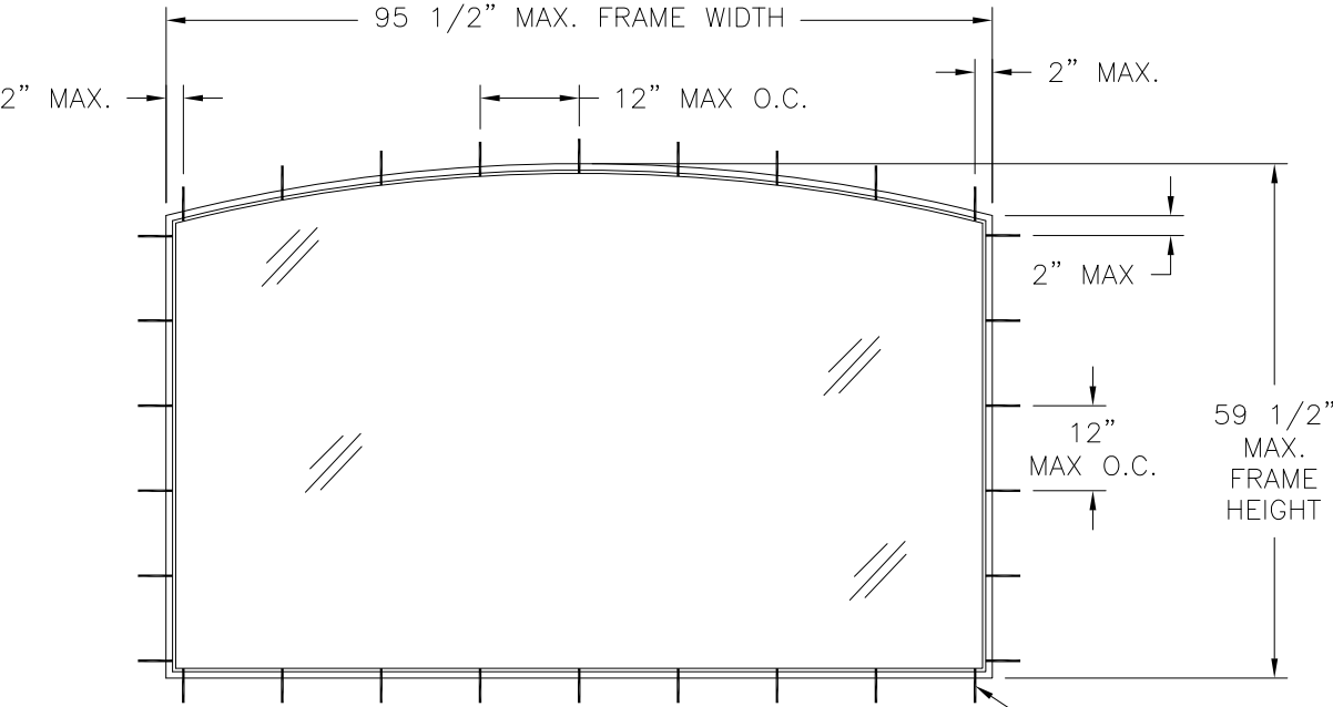
185 FIXED WINDOW DESIGNER EXTERIOR VIEW FLANGE & FINLESS INSTALLATION
