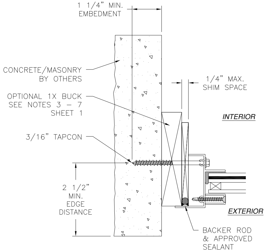
JAMB INSTALLATION DETAIL CONCRETE/MASONRY INSTALLATION
