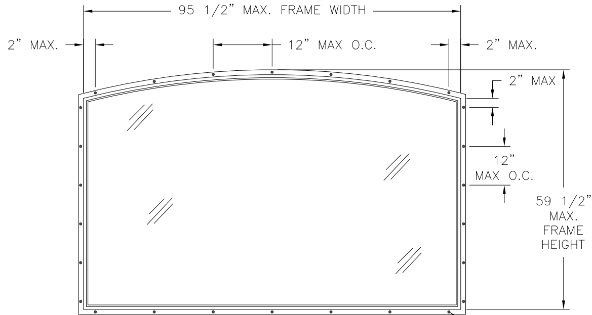
185 FIXED WINDOW DESIGNER EXTERIOR VIEW FIN INSTALLATION
