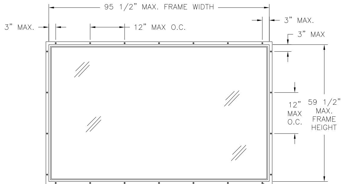
185 FIXED WINDOW EXTERIOR VIEW FIN INSTALLATION
