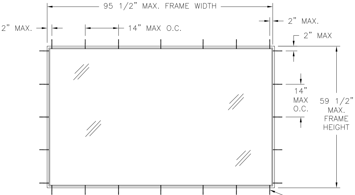
185 FIXED WINDOW EXTERIOR VIEW FLANGE & FINLESS INSTALLATION
