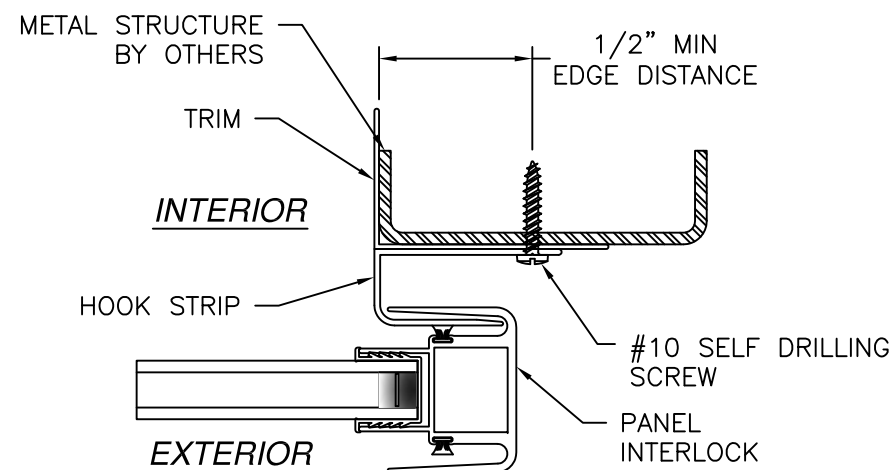
HOOK STRIP INSTALLATION METAL STRUCTURE
