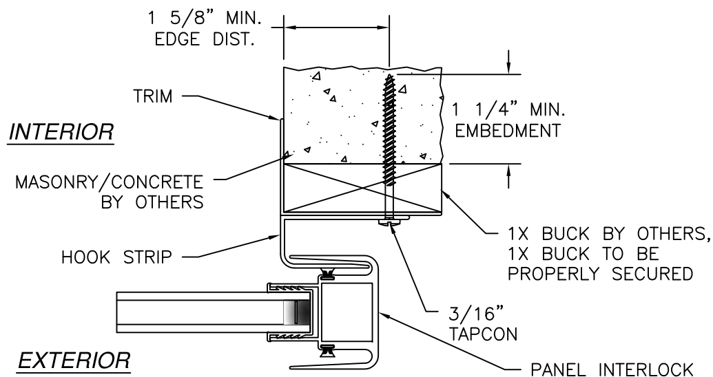
HOOK STRIP INSTALLATION MASONRY/CONCRETE
