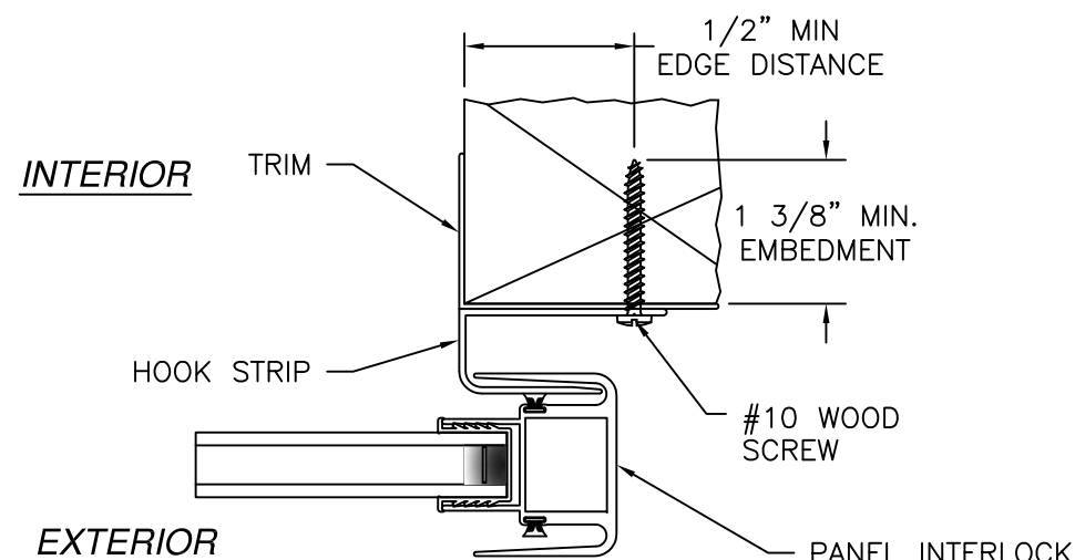
HOOK STRIP INSTALLATION 2X BUCK/WOOD FRAMING
