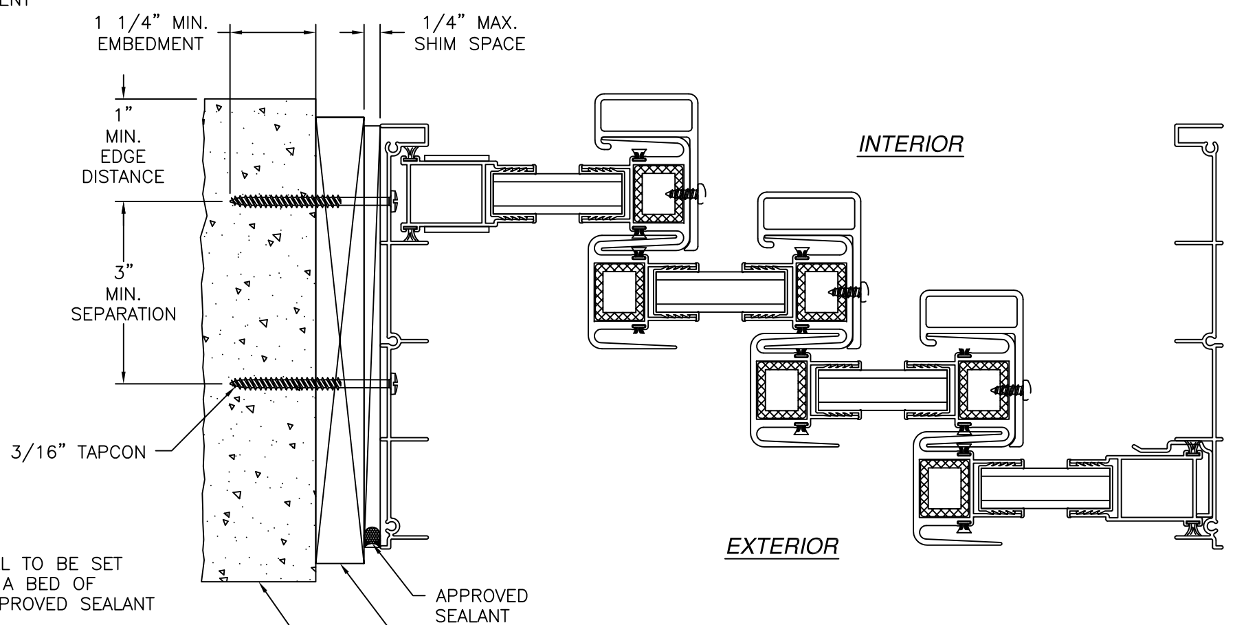
JAMB INSTALLATION DETAIL CONCRETE/MASONRY INSTALLATION
