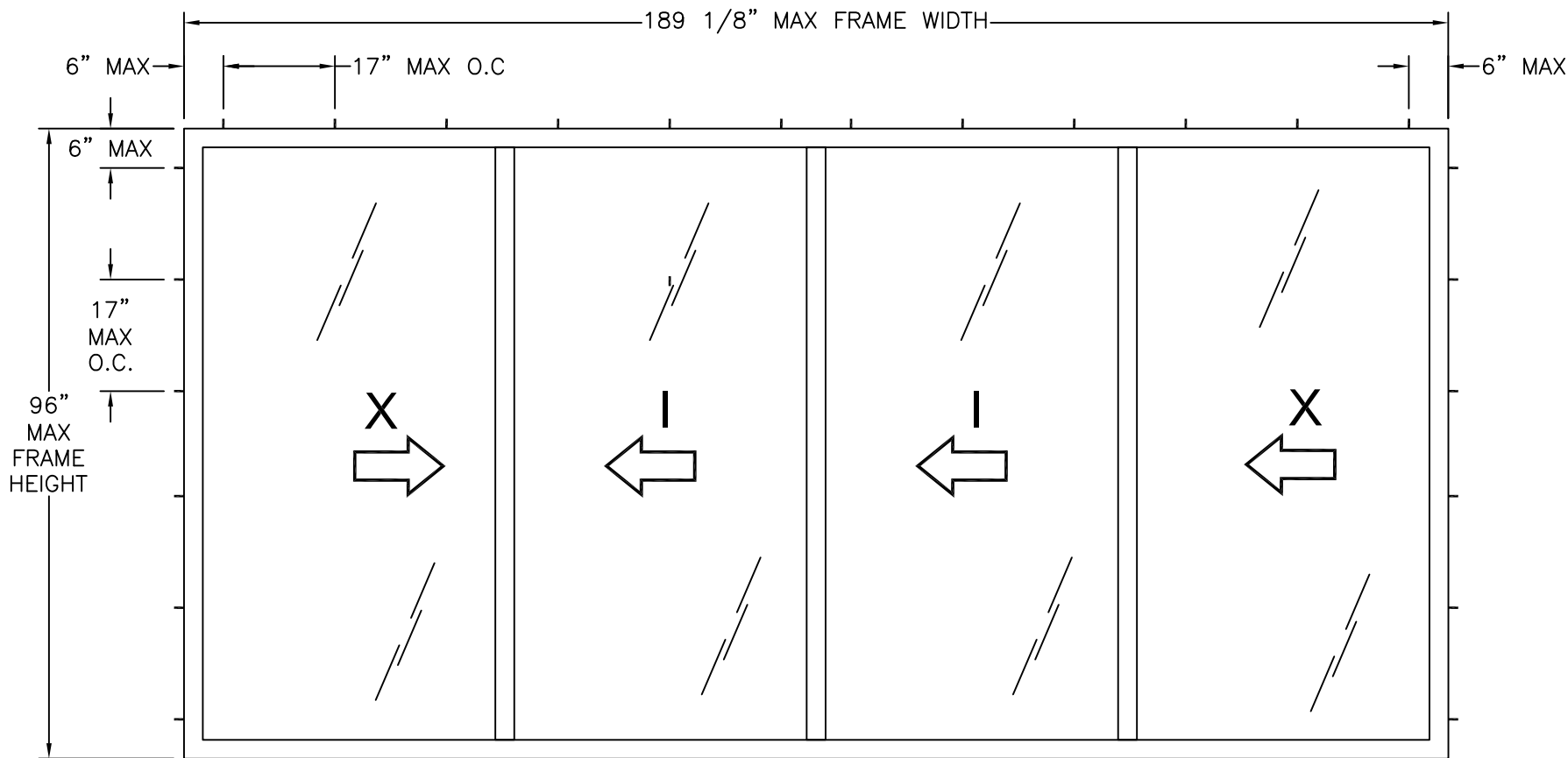
SERIES 440 XIIX SGD REINFORCED EXTERIOR VIEW
