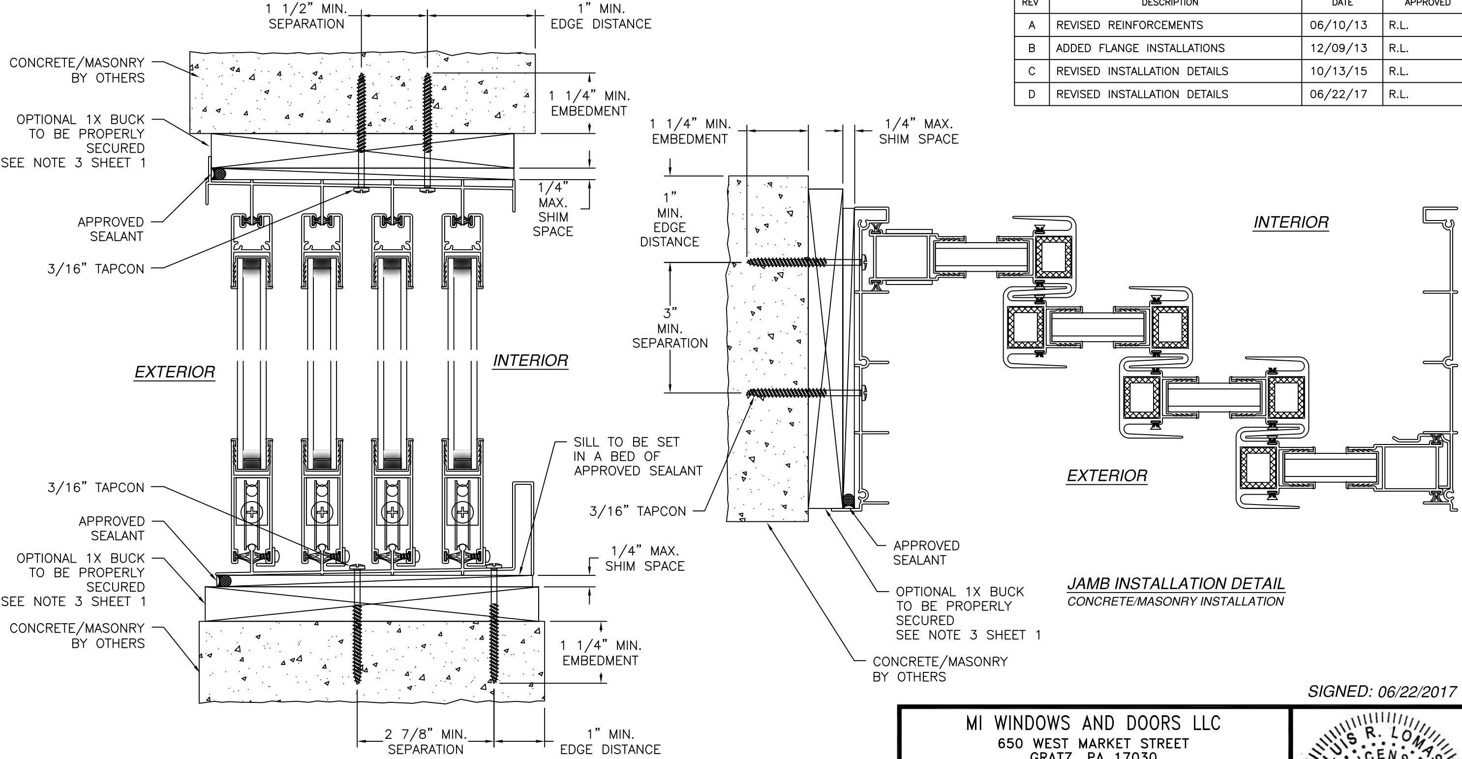
VERTICAL CROSS SECTION CONCRETE/MASONRY INSTALLATION
