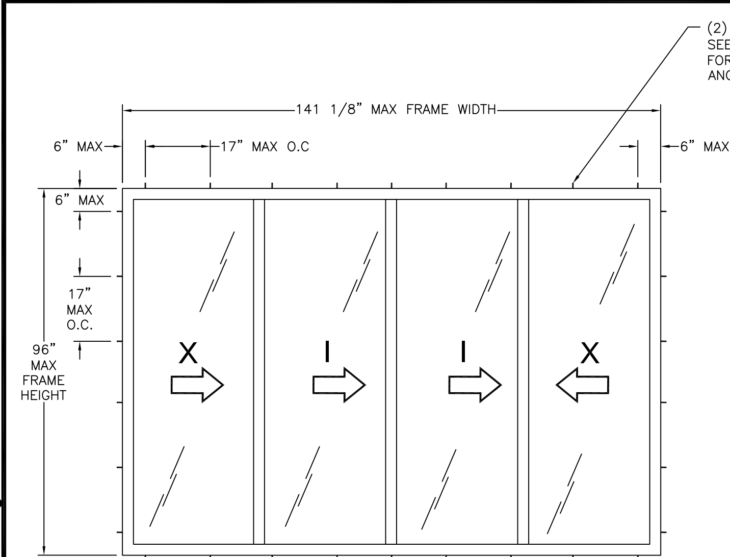
SERIES 440 XIIX SGD REINFORCED EXTERIOR VIEW
