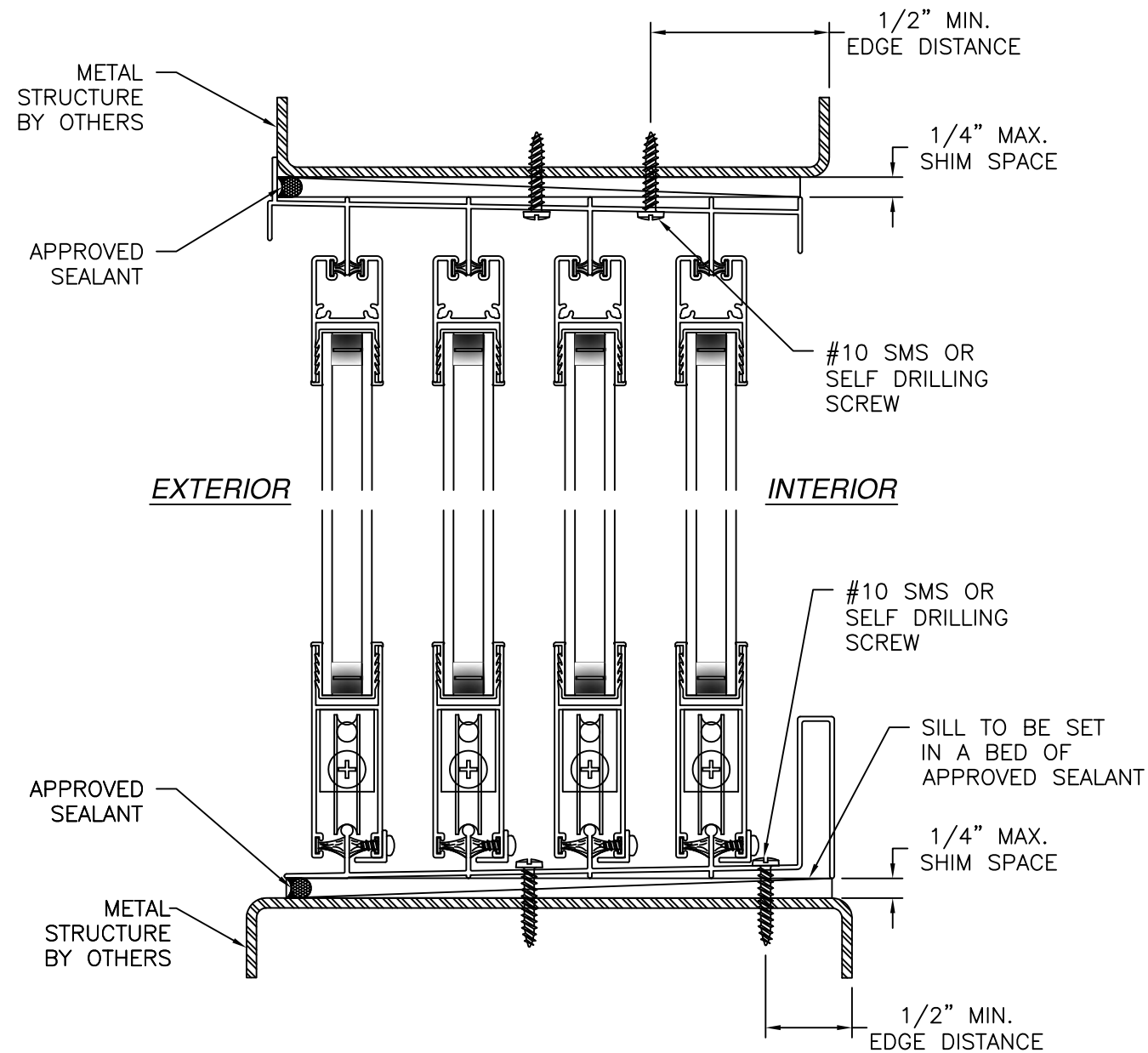
VERTICAL CROSS SECTION METAL STRUCTURE INSTALLATION
