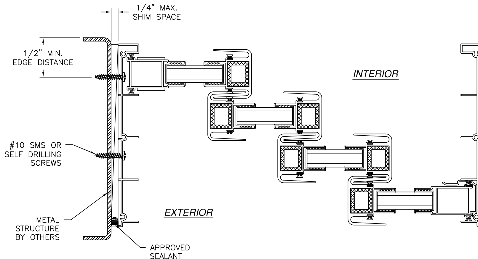
JAMB INSTALLATION DETAIL METAL STRUCTURE INSTALLATION
