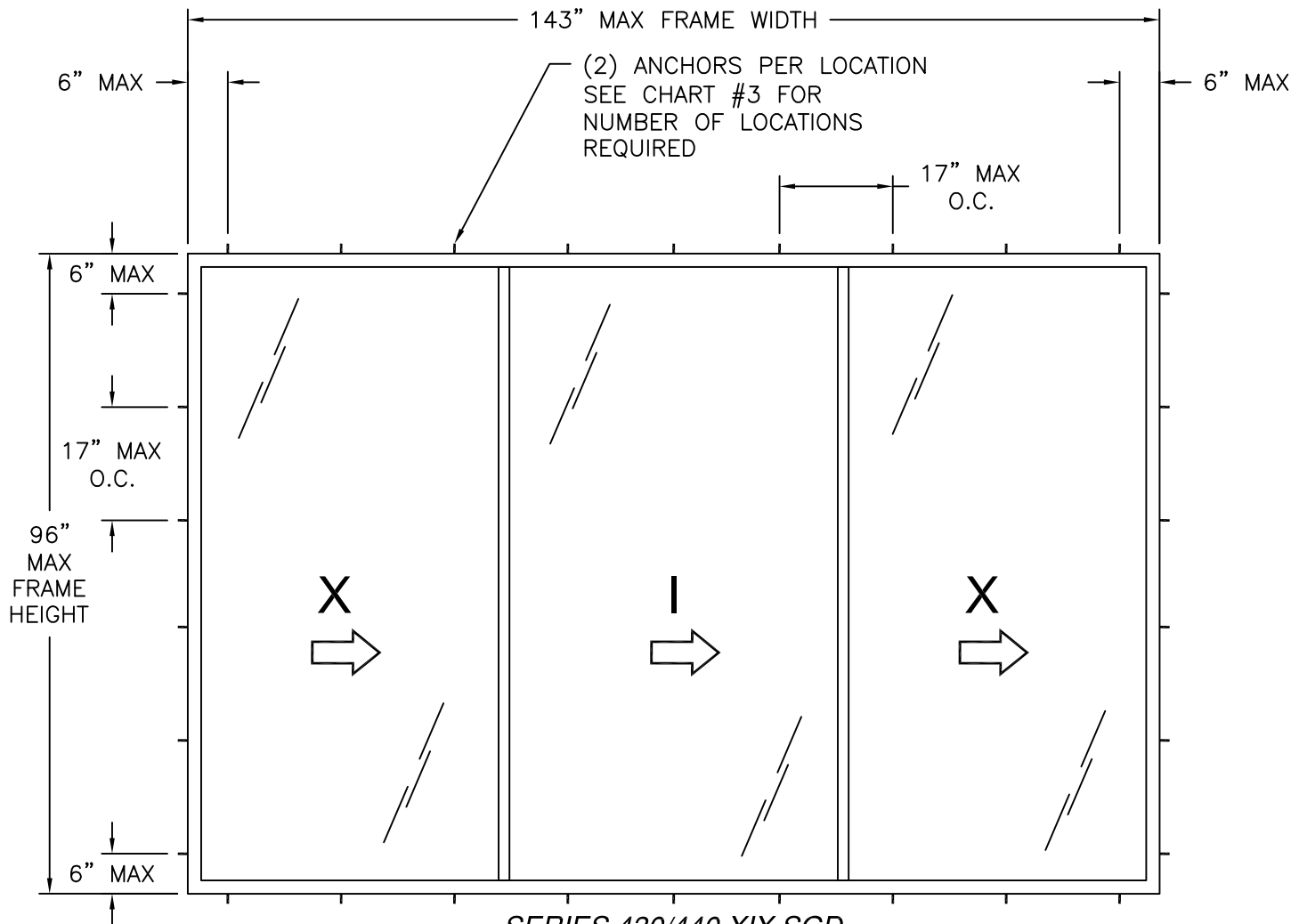
SERIES 430/440 XIX SGD EXTERIOR VIEW
