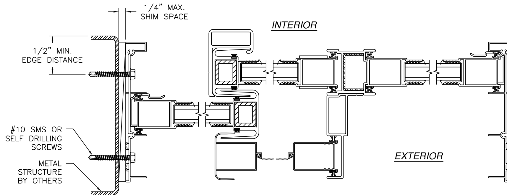
JAMB INSTALLATION DETAIL METAL STRUCTURE INSTALLATION
