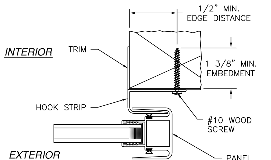
HOOK STRIP INSTALLATION 2X BUCK/WOOD FRAMING
