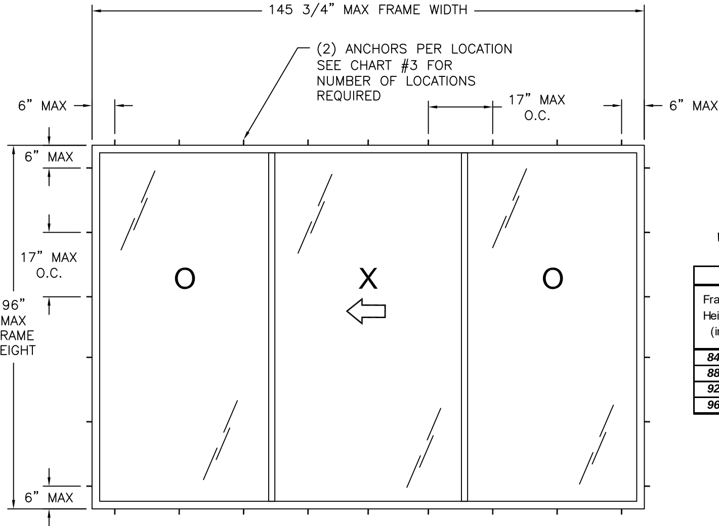
SERIES 420 SGD EXTERIOR VIEW
