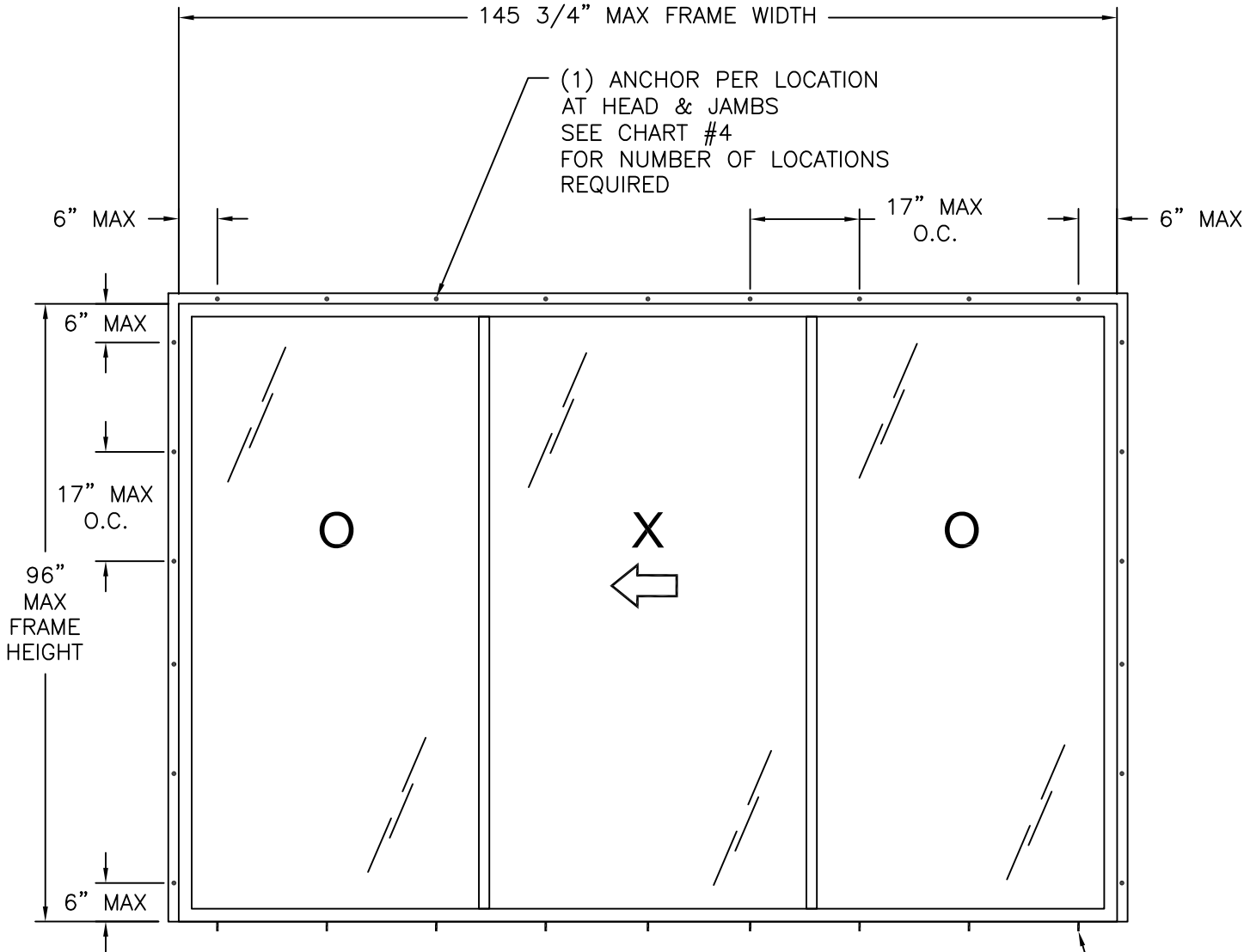
SERIES 420 SGD EXTERIOR VIEW
