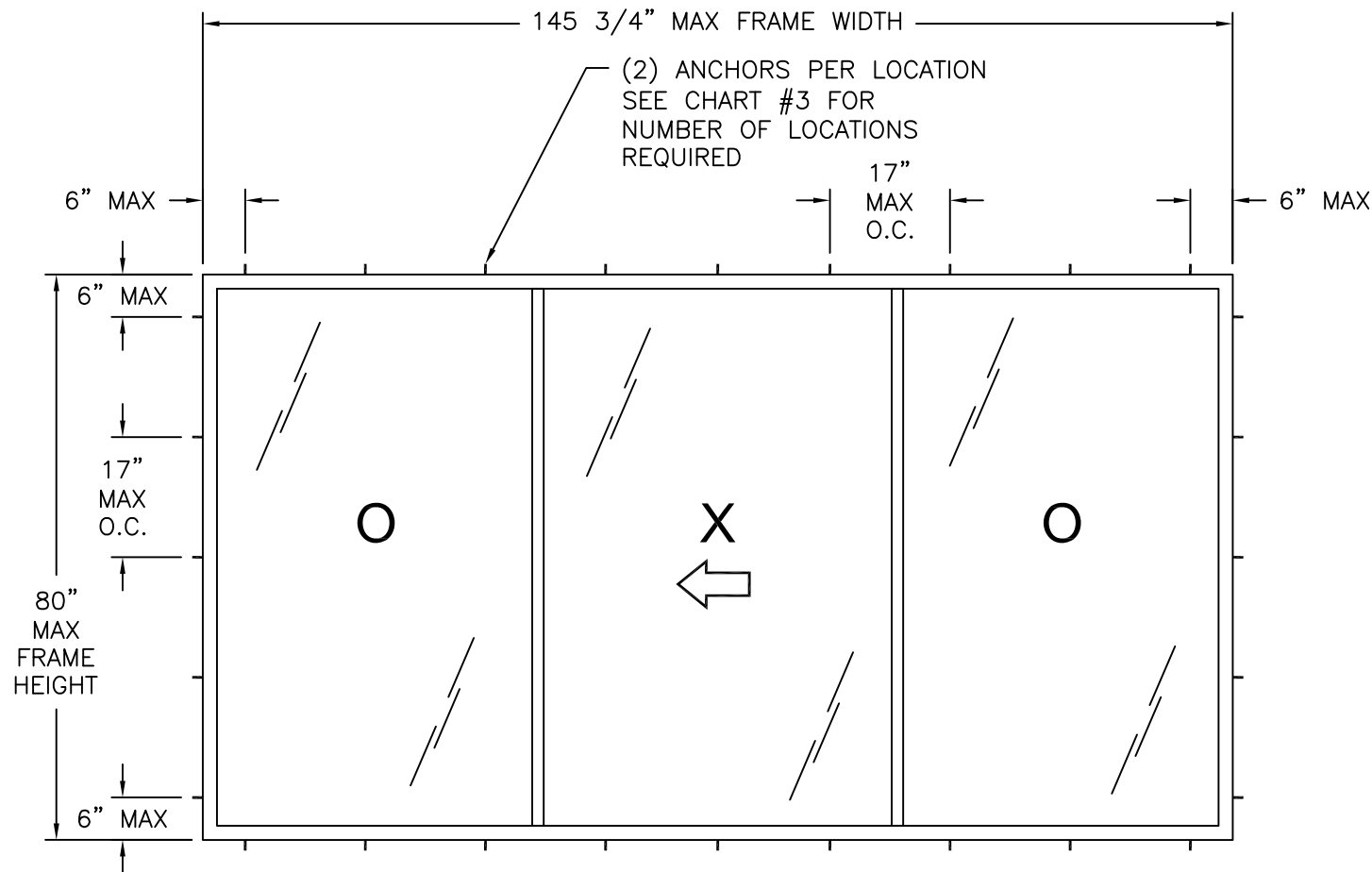
SERIES 420 OXO SGD EXTERIOR VIEW
