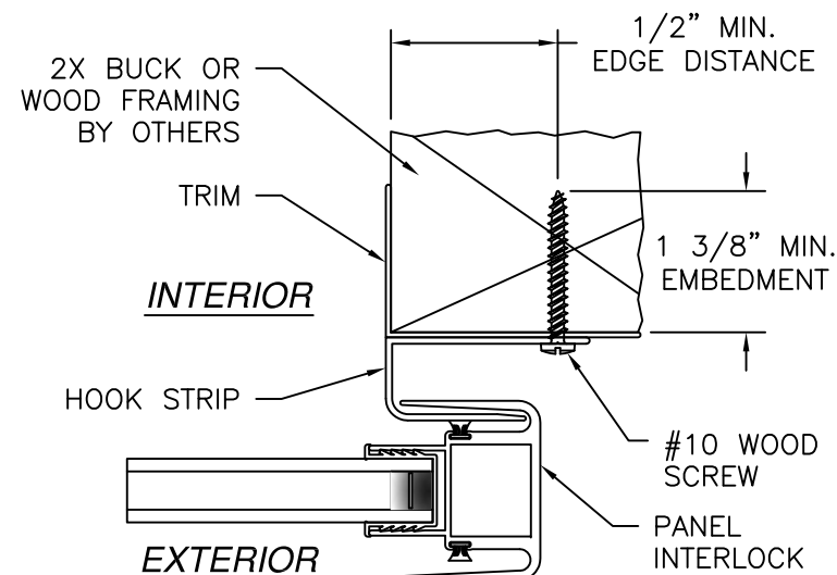
HOOK STRIP INSTALLATION 2X BUCK/WOOD FRAMING
