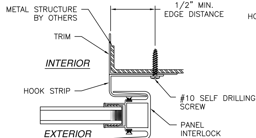
HOOK STRIP INSTALLATION METAL STRUCTURE
