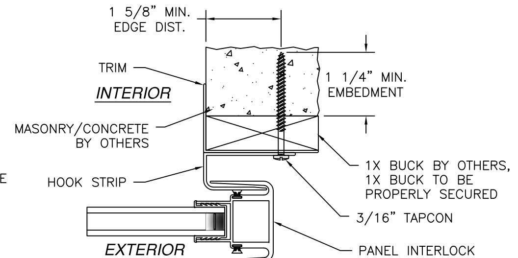
HOOK STRIP INSTALLATION MASONRY/CONCRETE
