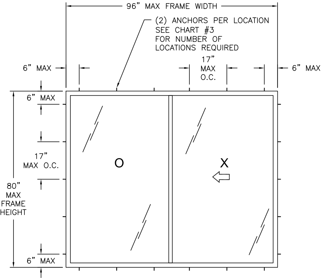
SERIES 420 SGD EXTERIOR VIEW
