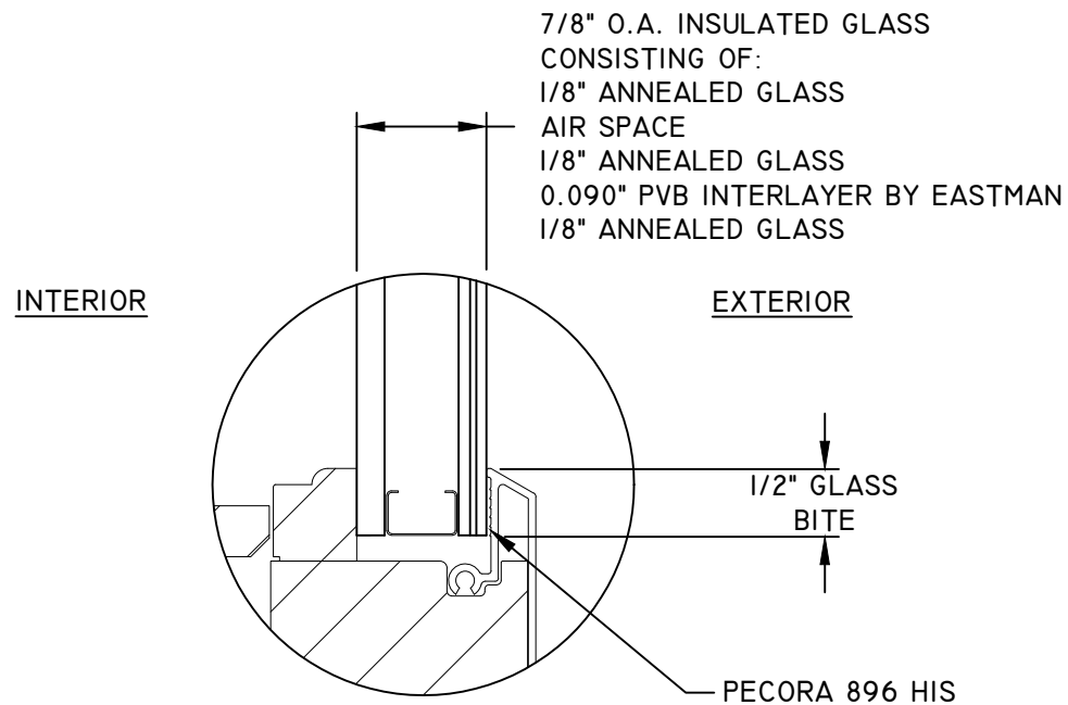
GLAZING DETAIL 1
