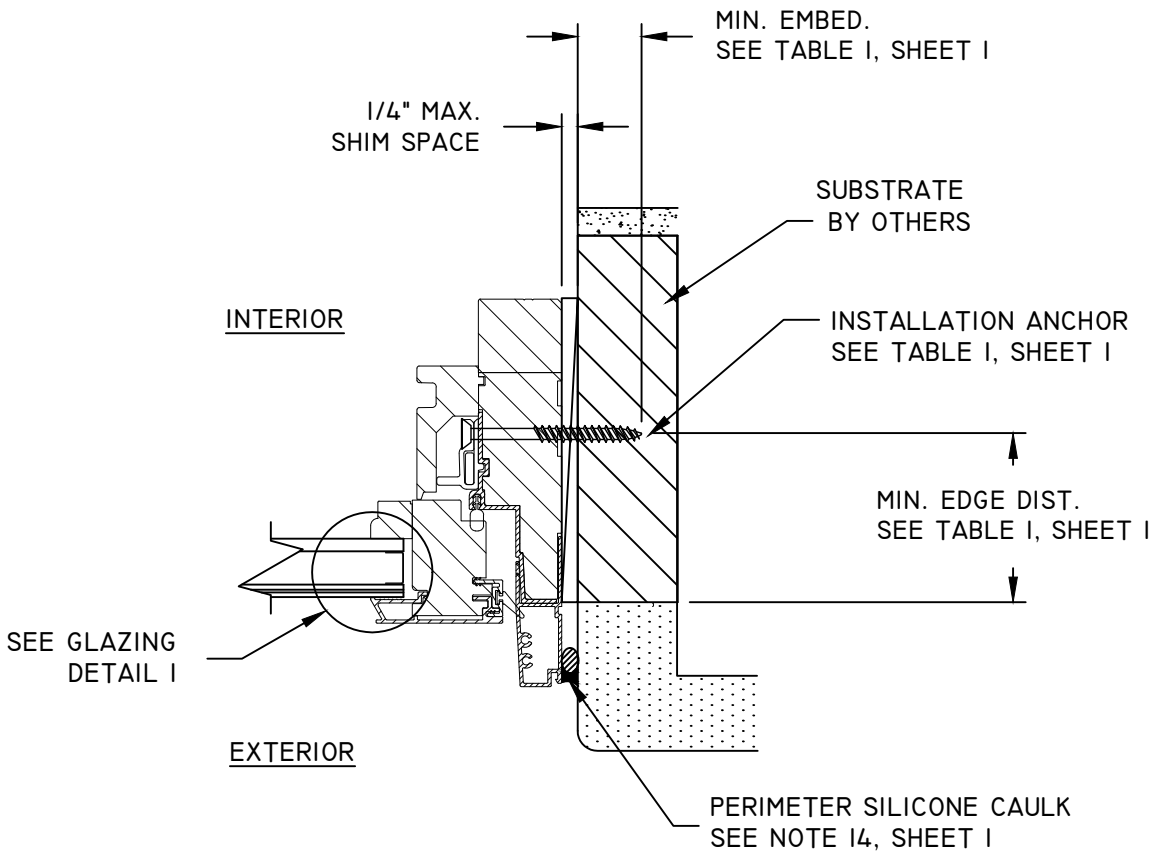
F 4 HORIZONTAL SECTION JAMB FRAME INSTALLATION
