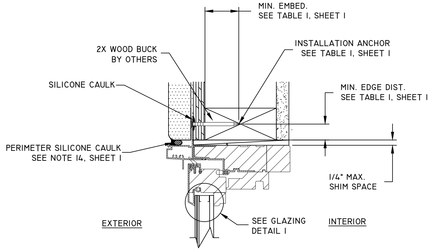
B 3 VERTICAL SECTION HEAD FIN INSTALLATION
