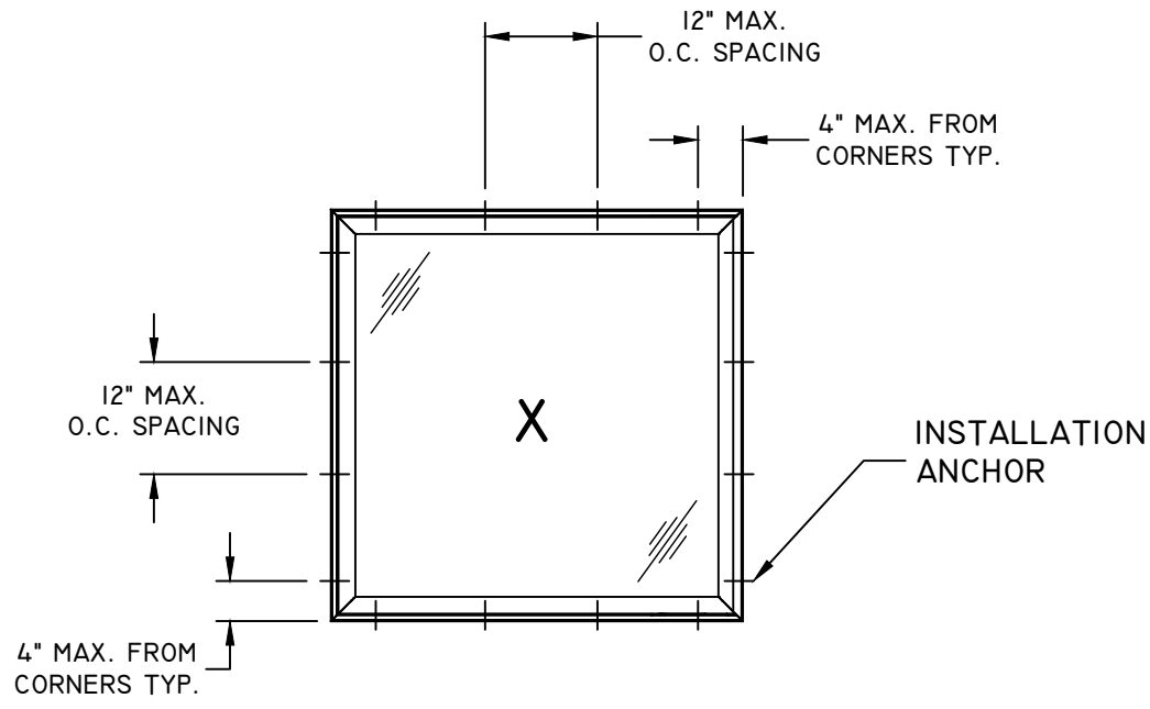
ANCHOR LAYOUT FRAME INSTALLATION
