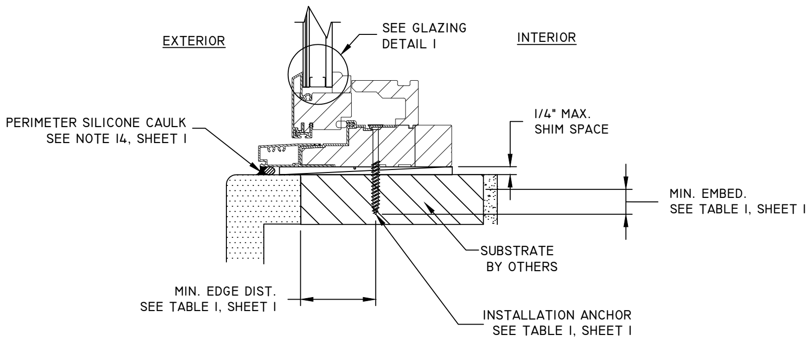
D 4 VERTICAL SECTION SILL FRAME INSTALLATION
