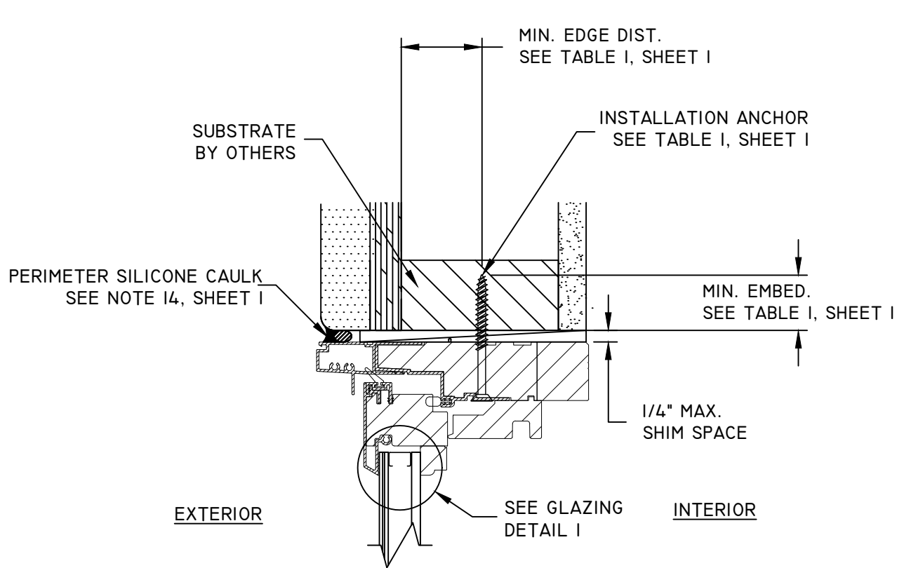
E 4 VERTICAL SECTION HEAD FRAME INSTALLATION
