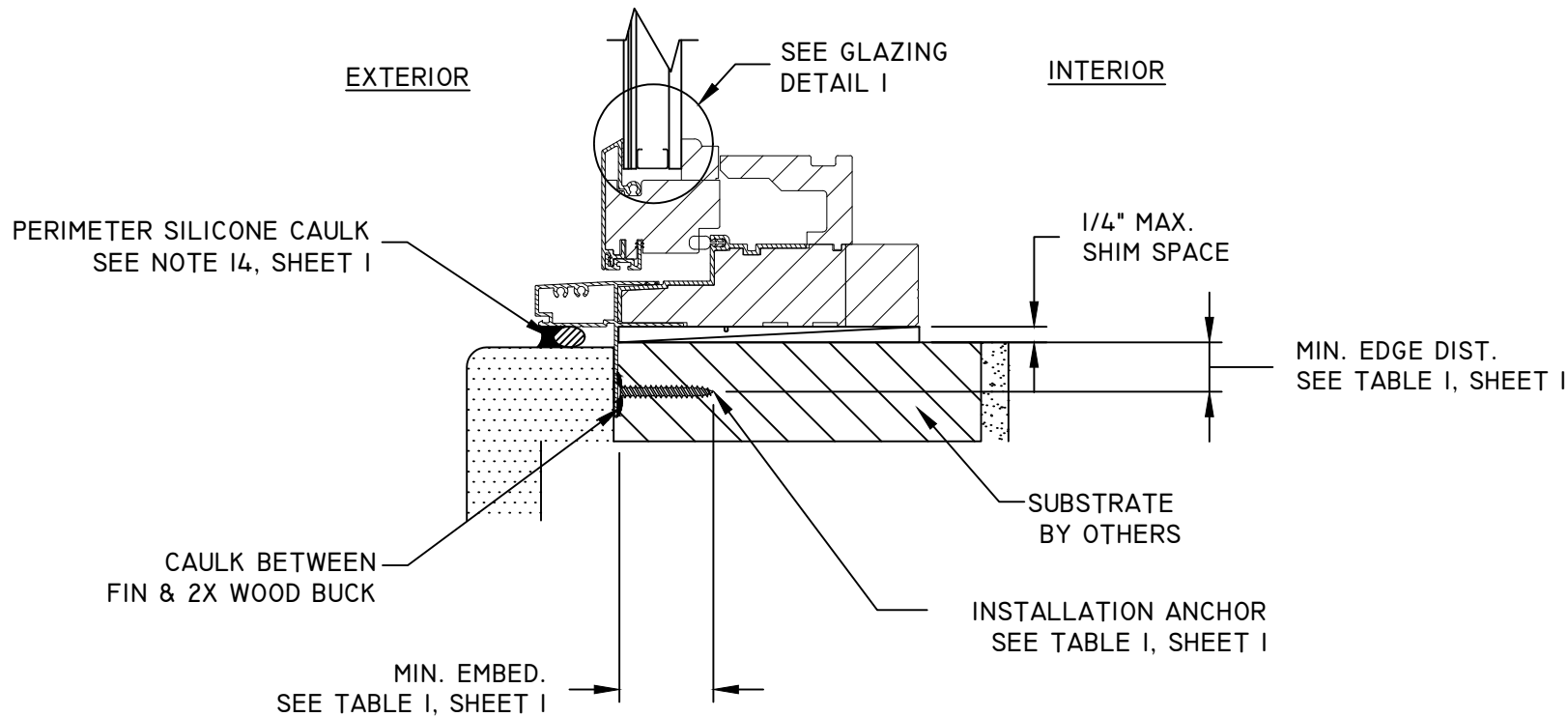
A 3 VERTICAL SECTION SILL FIN INSTALLATION
