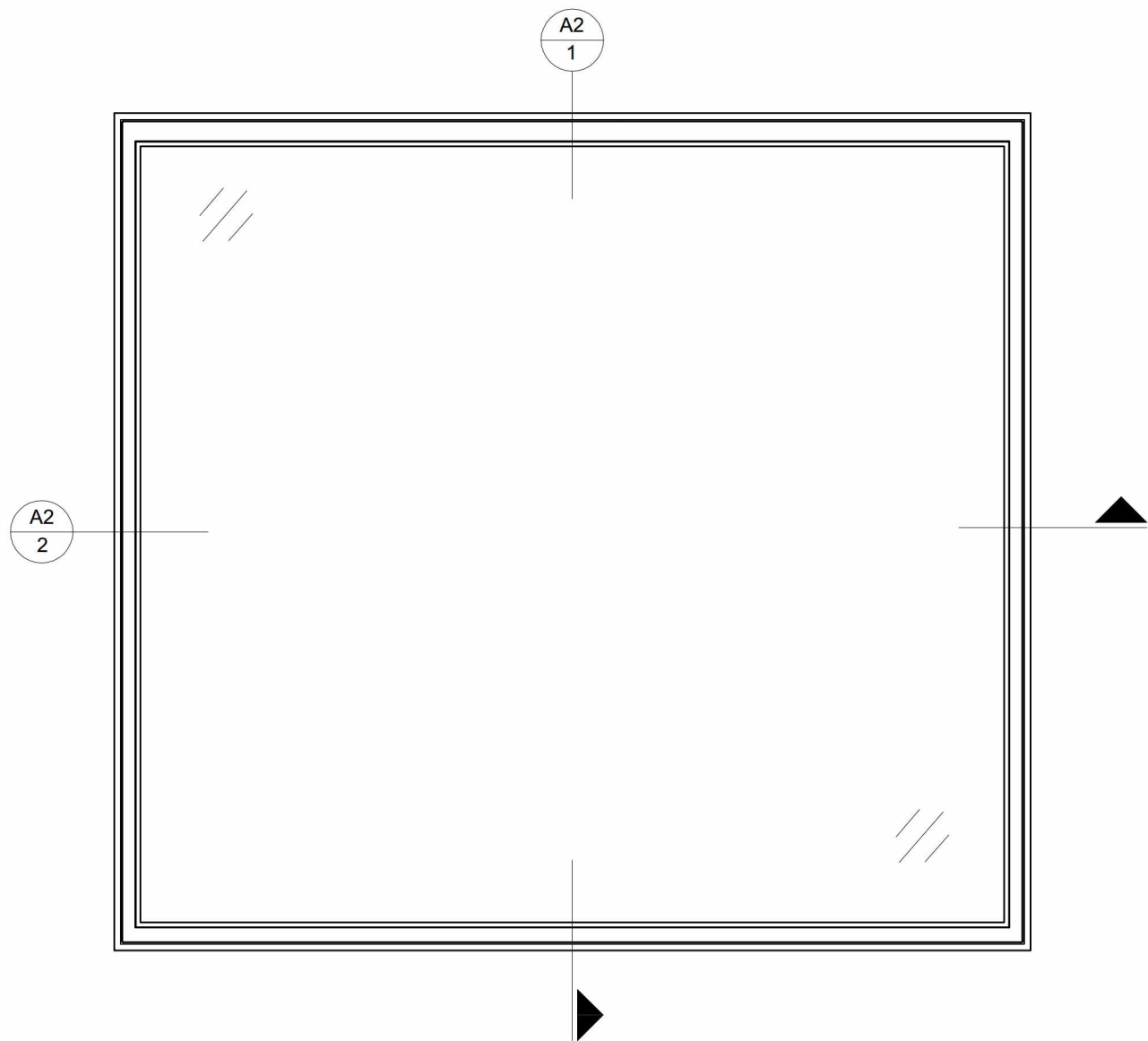
A1 1 ELEVATION - WOOD FIXED CASEMENT SCALE: 1:1
