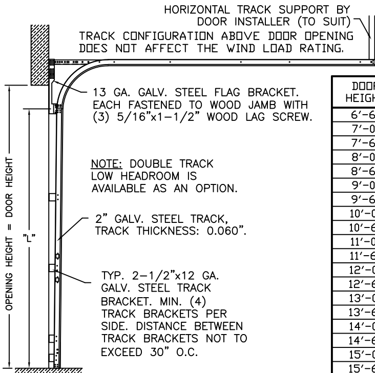
TRACK CONFIGURATION
