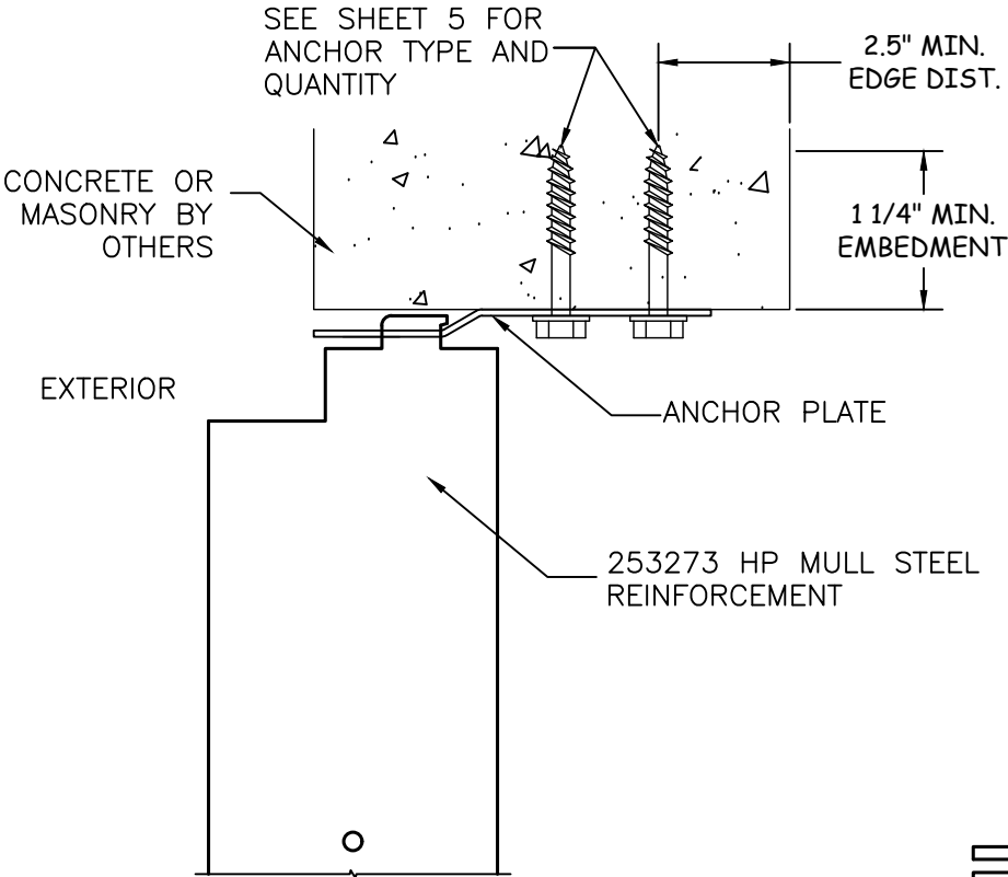
A 3 VERTICAL SECTION (MASONRY, ANCHOR PLATE)
