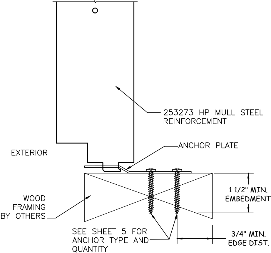
C 3 VERTICAL SECTION (WOOD, ANCHOR PLATE)
