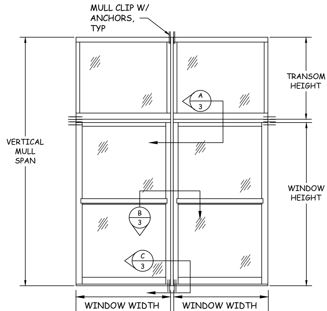
VERTICAL MULLION FOR TWIN WINDOW WITH TRANSOM SEE CHARTS ON SHEET 5 FOR DESIGN PRESSURES AND ANCHOR SCHEDULE
