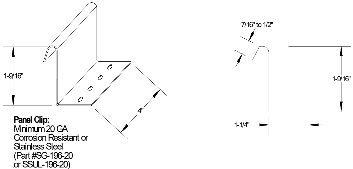
Typical Panel Clip Profile
