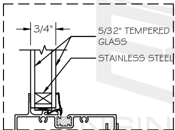
(G1) GLASS DETAIL (NON IMPACT)
