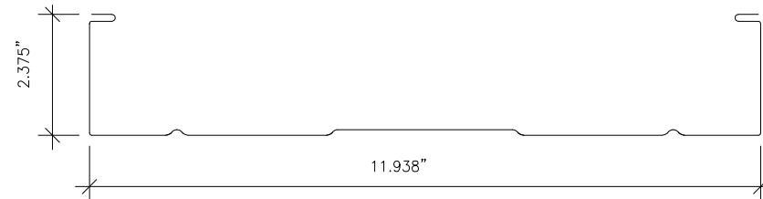
PANEL SECTION (MIN 22 GA.)
