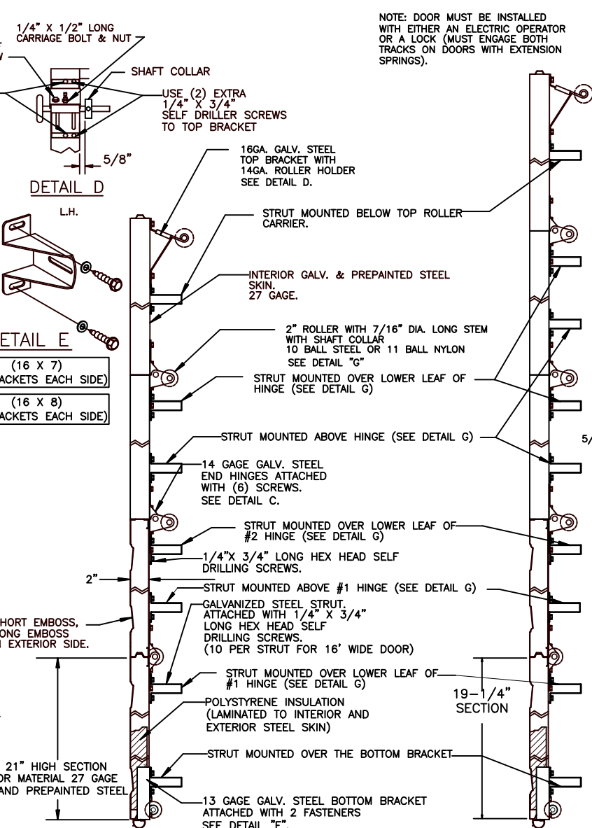
SECTION A-A 4 SECTION SECTION C-C 5 SECTION
