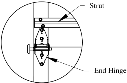
Strut above hinge Detail B
