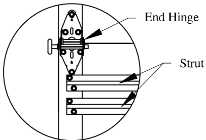
Additional Strut below hinge
