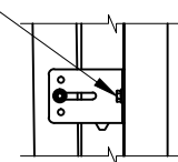
Track Bracket (.102) galvanized steel track bracket attached to wood jamb with one 5/16" x 1-5/8" wood lag screw per bracket and attached to vertical track with one 1/4" x 5/8" track bolt and nut or two 1/4" x 11/32" rivets.
