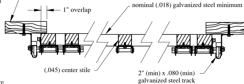
End Hinge galvanized steel attached with six 1/4\"/>
