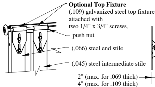
End Stile (.066) steel end stile
