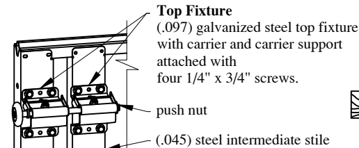
End Stile (.066) steel end stile
