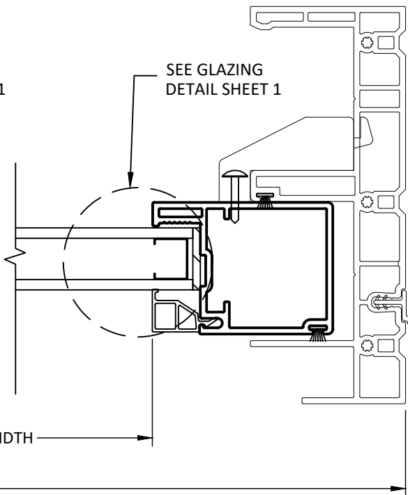
F 4 HORIZONTAL SECTION SNAP ON FLANGE-FRAME INSTALLATION
