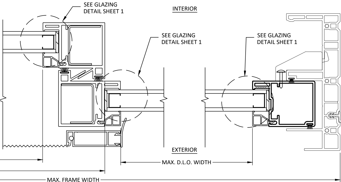
E 4 HORIZONTAL SECTION MEETING RAILS
