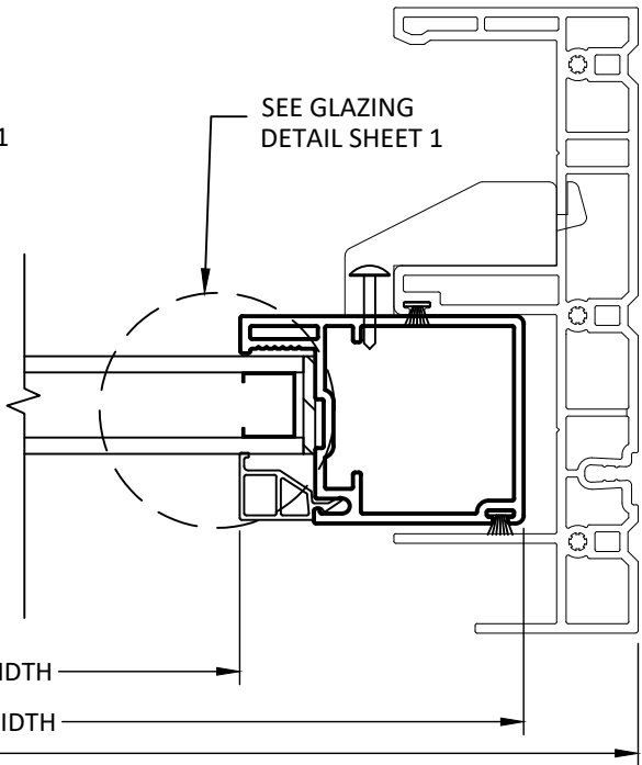
C 4 HORIZONTAL SECTION THROUGH FRAME INSTALLATION
