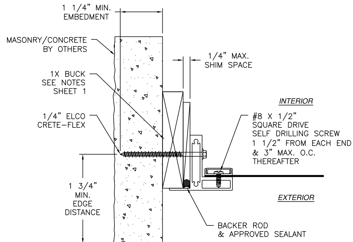
JAMB INSTALLATION DETAIL MASONRY/CONCRETE INSTALLATION JAMB SHOWN, HEAD AND SILL SIMILAR
