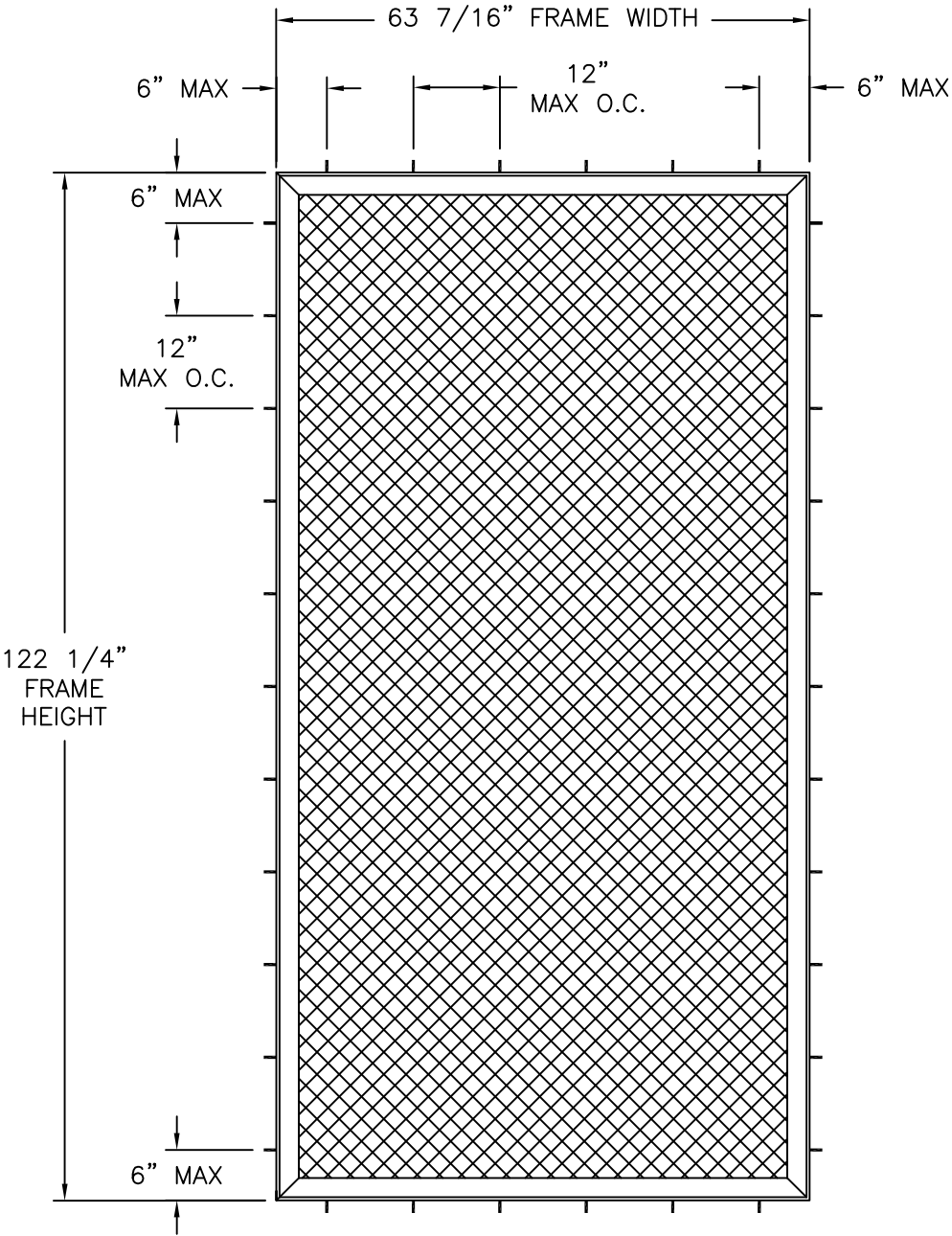
SERIES 950 PATIO SCREEN ENCLOSURE EXTERIOR VIEW
