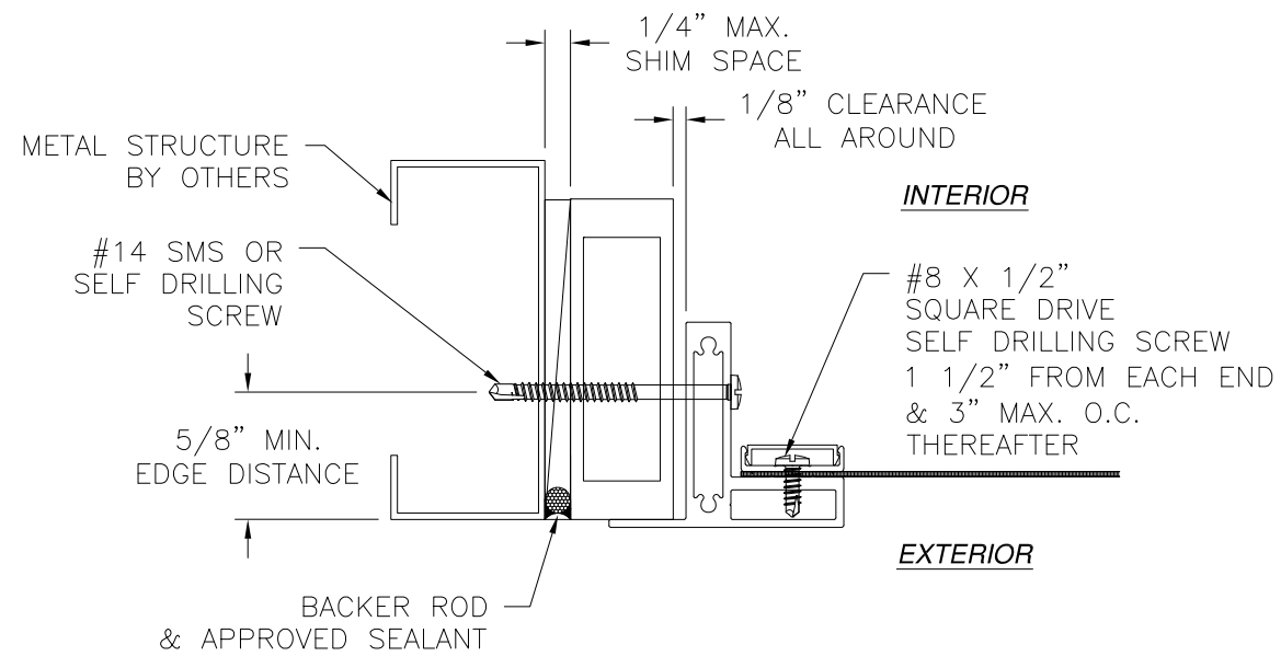
JAMB INSTALLATION DETAIL METAL STRUCTURE INSTALLATION JAMB SHOWN, HEAD AND SILL SIMILAR
