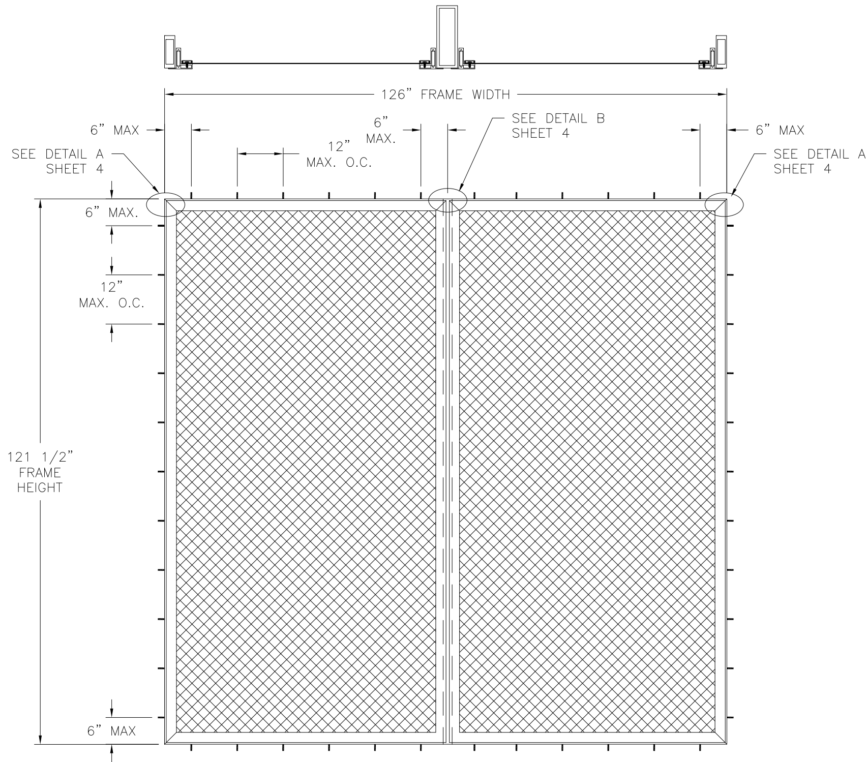
SERIES 950 PATIO SCREEN ENCLOSURE EXTERIOR VIEW
