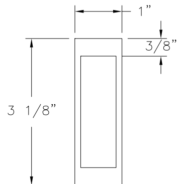
RECTANGULAR TUBE (54314) ALUMINUM 6005-T5 (1/8" THICK)
