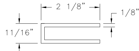
INSIDE U-CLIP (52-63-11886) ALUMINUM 6063-T5
