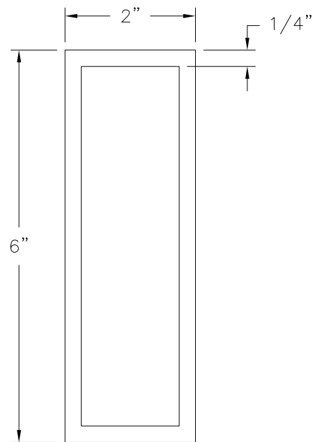
CENTER MULLION (610068) ALUMINUM 6005-T5 (1/4" THICK)
