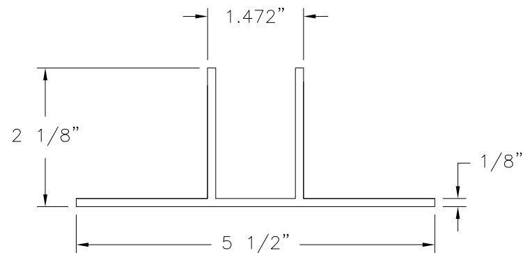
CLIP INSERT (52-63-8746) ALUMINUM 6063-T5 (1/8" THICK)
