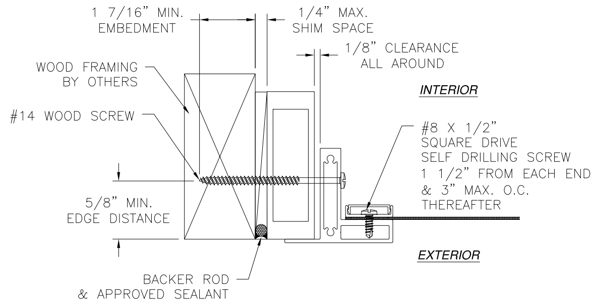
JAMB INSTALLATION DETAIL WOOD FRAMING OR 2X BUCK INSTALLATION JAMB SHOWN, HEAD AND SILL SIMILAR
