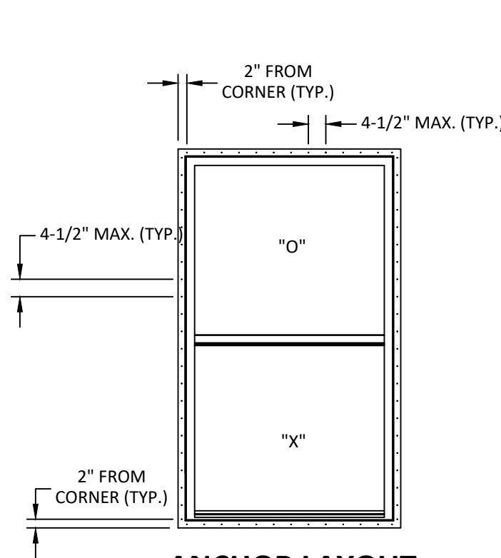
ANCHOR LAYOUT NAIL FIN
