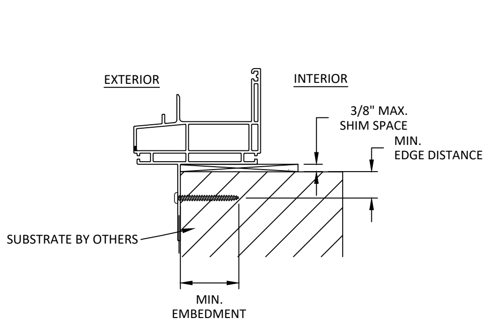
A 5 ANCHOR DETAIL NAIL FIN (SILL)
