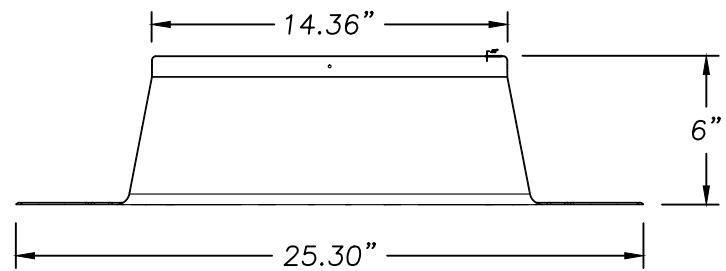
12 FLASHING 14" NO PITCH 6" ALUMINIZED STEEL EDSS T1-25 .028" THICK
