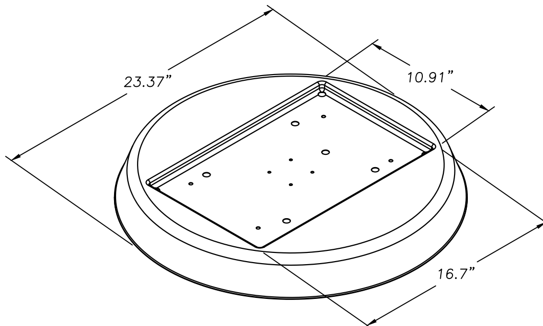
3 TOP PANEL SS 14" BLACK ALUMINIZED STEEL EDSS T1-25 .028" THICK
