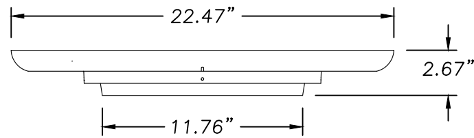
2 FAN GRILL, SOLAR STAR 14" POLYPROPYLENE .120" THICK
