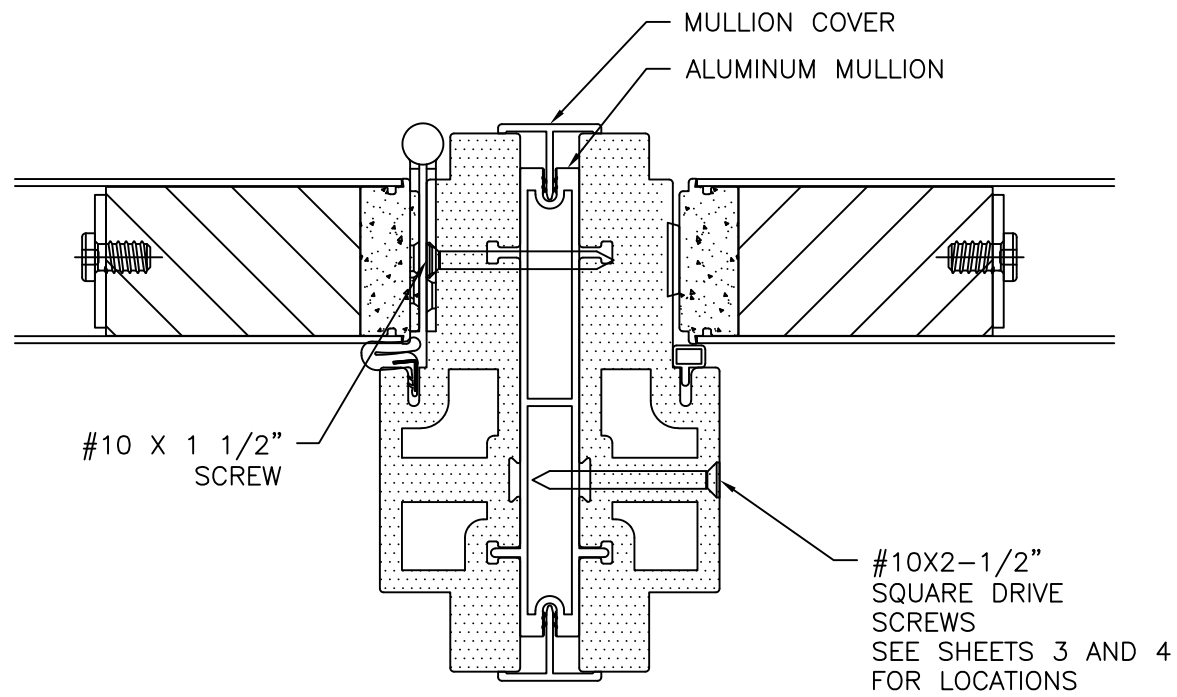
MULLION DETAIL
