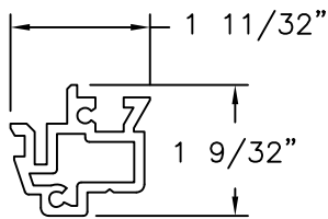
REINFORCEMENT (A) ALUMINUM
