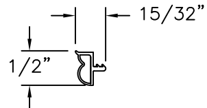
WEATHER STRIP (C) EPDM
