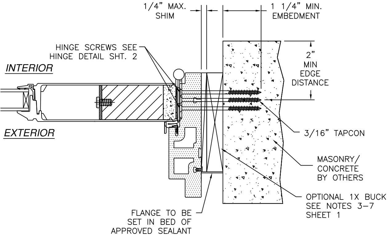
DOOR HORIZONTAL CROSS SECTION MASONRY/CONCRETE INSTALLATION
