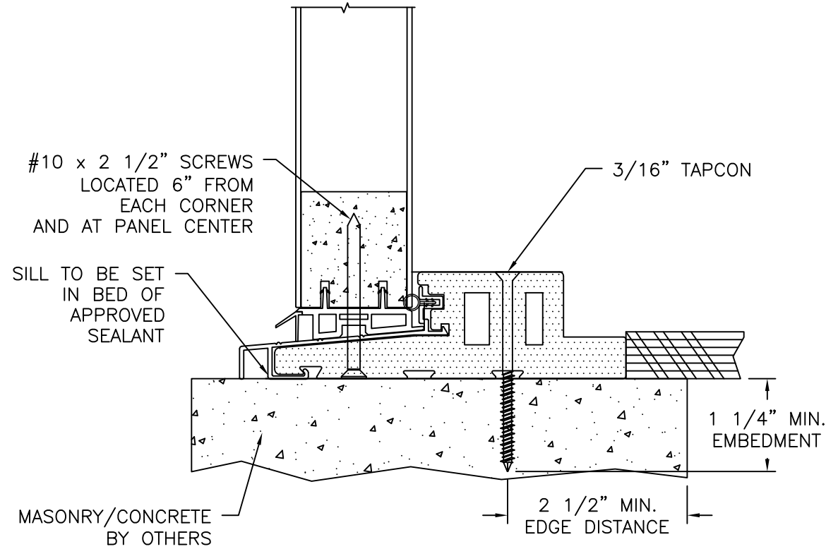
SIDELITE VERTICAL CROSS SECTION MASONRY/CONCRETE INSTALLATION
