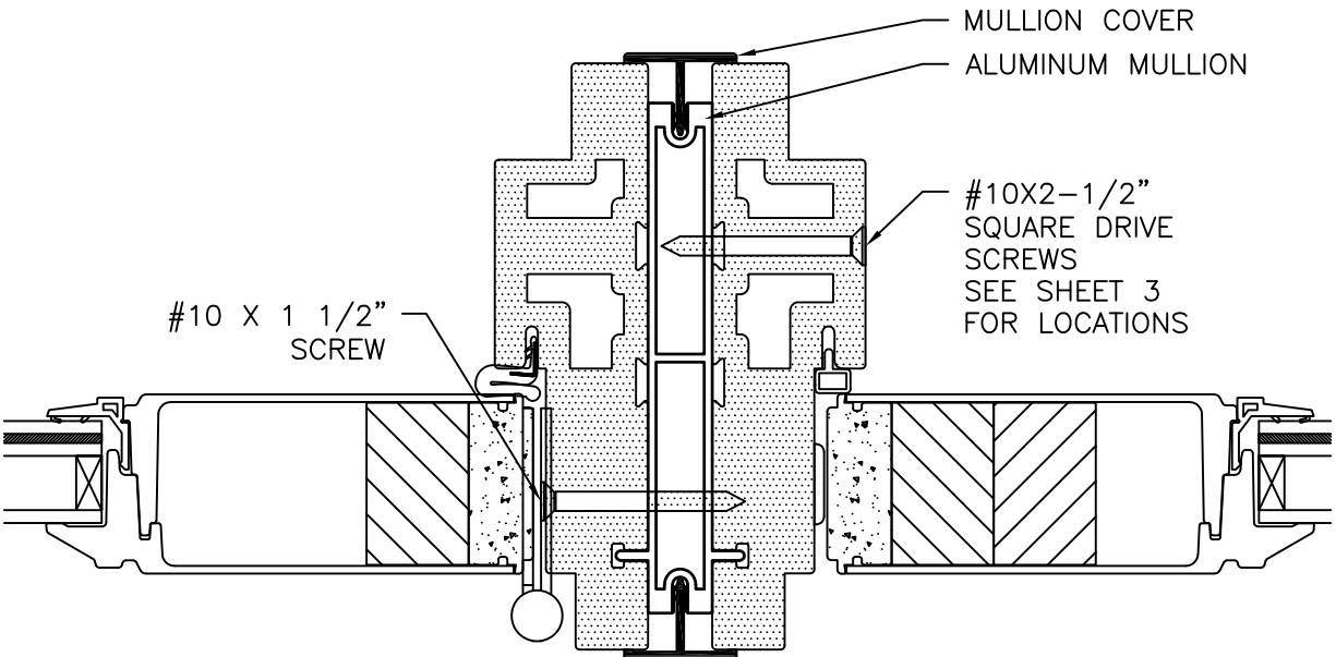
MULLION DETAIL
