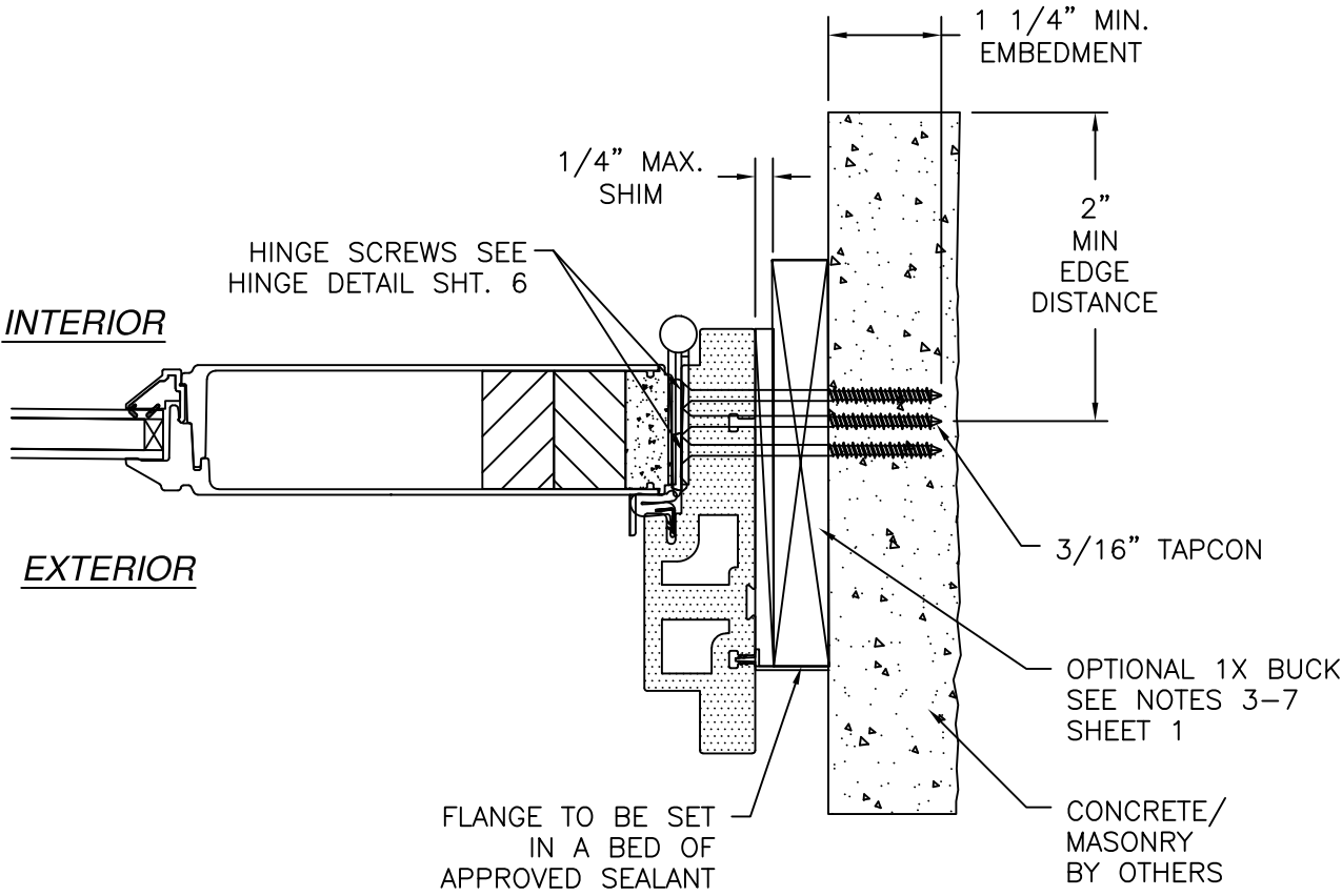
DOOR HORIZONTAL CROSS SECTION CONCRETE/MASONRY INSTALLATION
