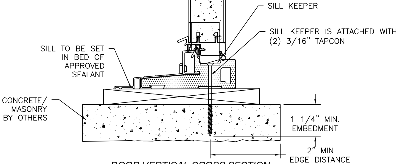
DOOR VERTICAL CROSS SECTION CONCRETE/MASONRY INSTALLATION
