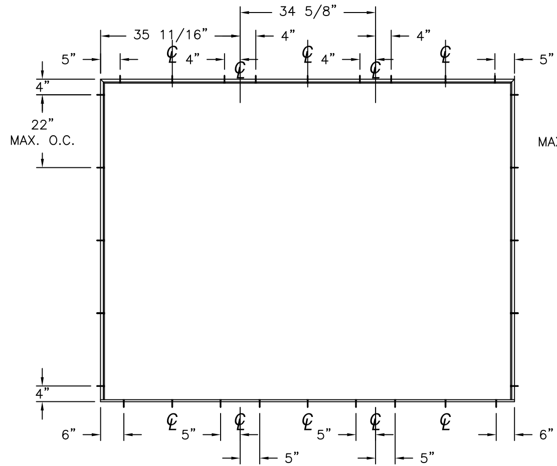
ANCHORING LAYOUT FOR OXO, XXO AND OXX
