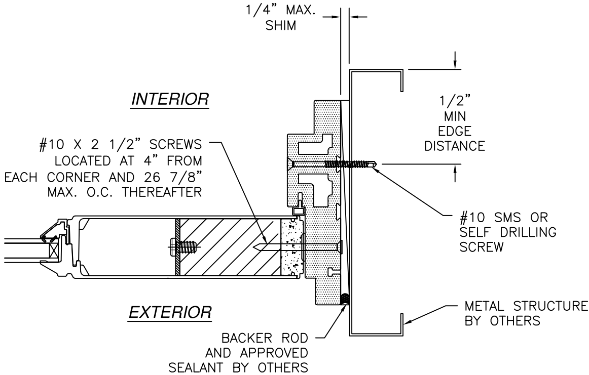
SIDELITE HORIZONTAL CROSS SECTION METAL STRUCTURE INSTALLATION
