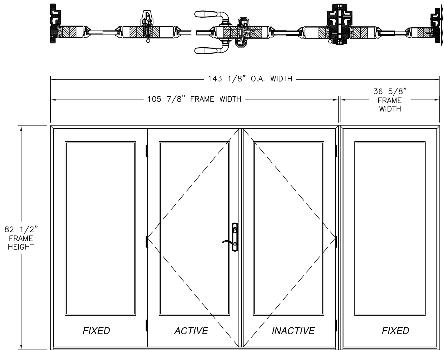
OUT-SWING ENTRANCE DOUBLE DOOR W/ SIDELITES EXTERIOR VIEW
