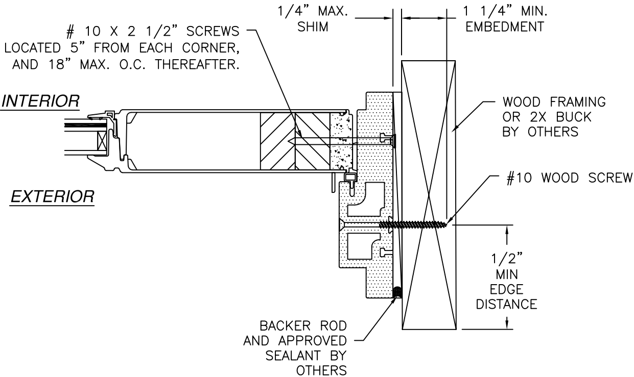
SIDELITE HORIZONTAL CROSS SECTION WOOD FRAMING OR 2X BUCK INSTALLATION
