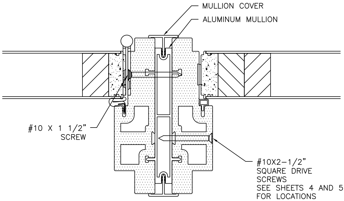
MULLION DETAIL
