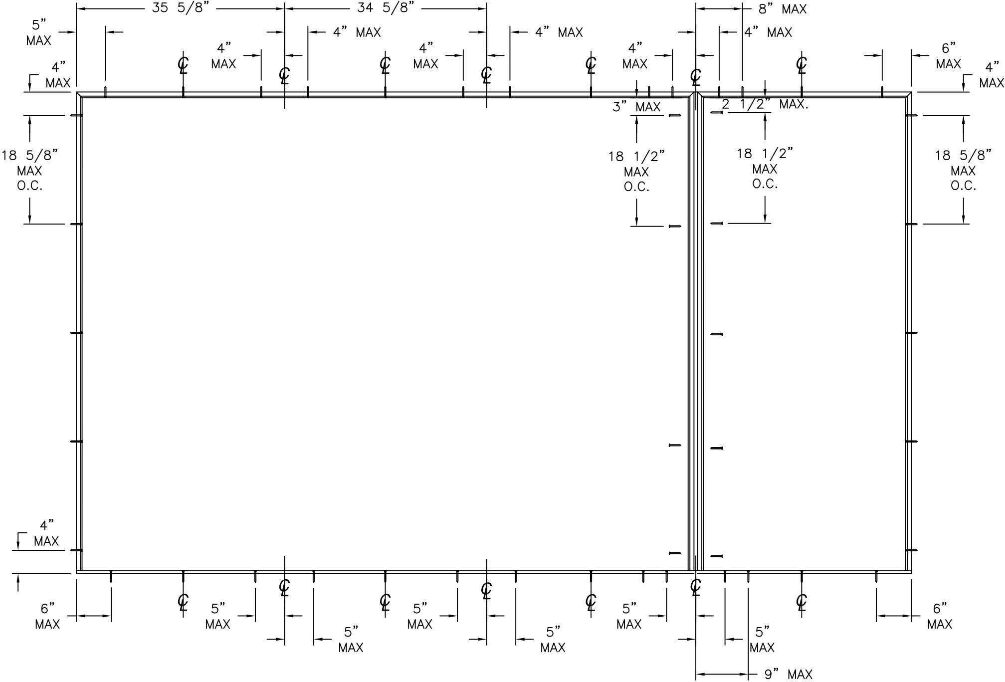
ANCHORING LAYOUT
