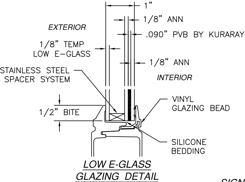
MINI-BLIND GLAZING DETAIL
