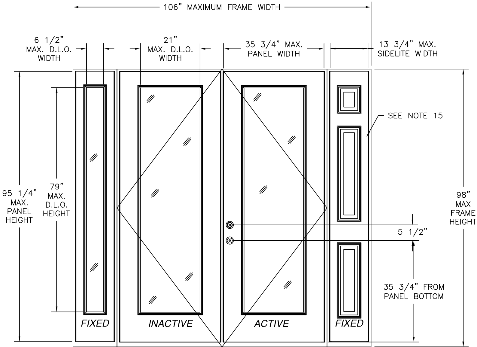
8' DISTINCTION IS FIBERGLASS GLAZED PATIO DOUBLE DOOR W/ SIDELITES EXTERIOR VIEW
