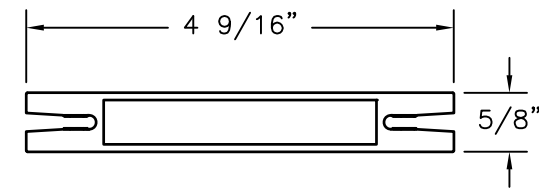
MULLION REINFORCEMENT EXTRUDED ALUMINUM 6063-T6 .078" THICK
