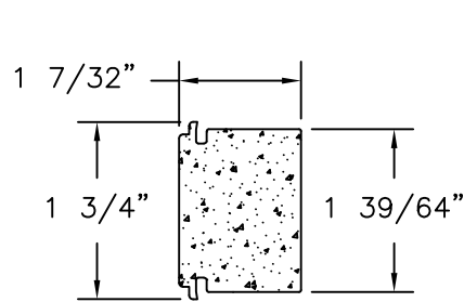
1 7/32" STILE FOAM PVC
