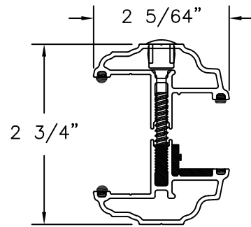
ODL HURRICANE LITE FRAME EXTRUDED ALUMINUM 6063-T6 .065" THICK
