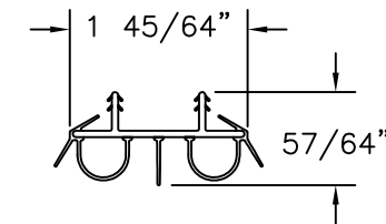
ENDURA DOOR BOTTOM EXTRUDED PVC .061" THICK
