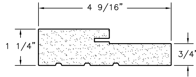
4 9/16" HEAD AND JAMB EXTRUDED PVC COMPOSITE
