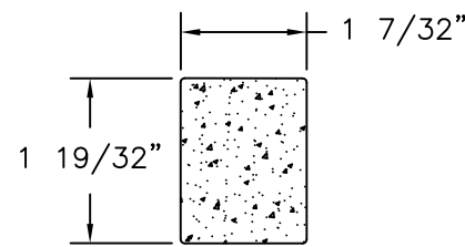
TOP AND BOTTOM RAIL FOAM PVC
