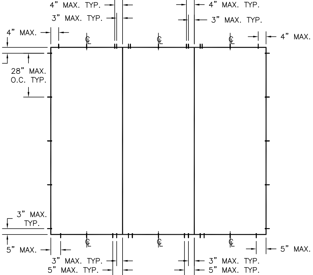
SINGLE W/SIDELITES, DOUBLE W/SIDELITE OR TRIPLE FIXED
