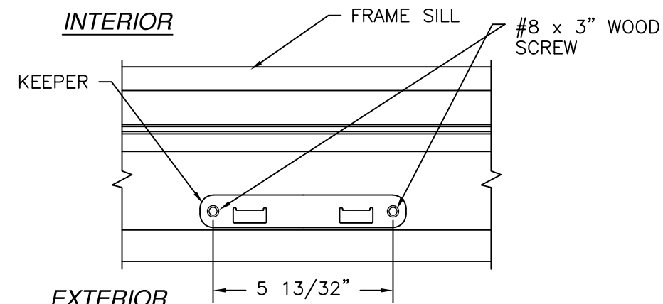
SILL KEEPER DETAIL
