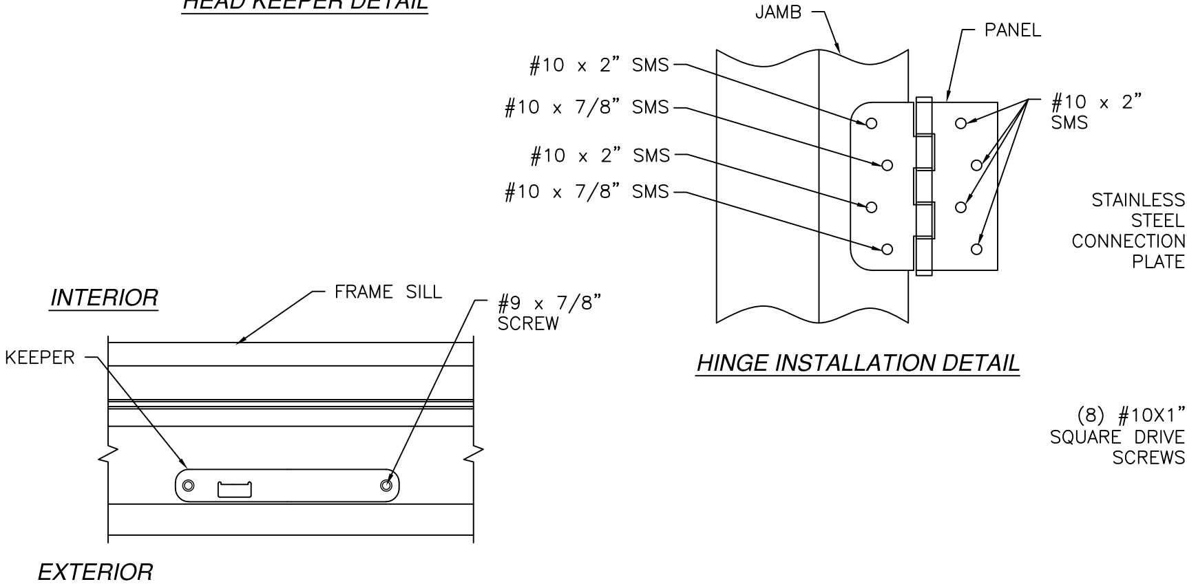
SILL KEEPER DETAIL
