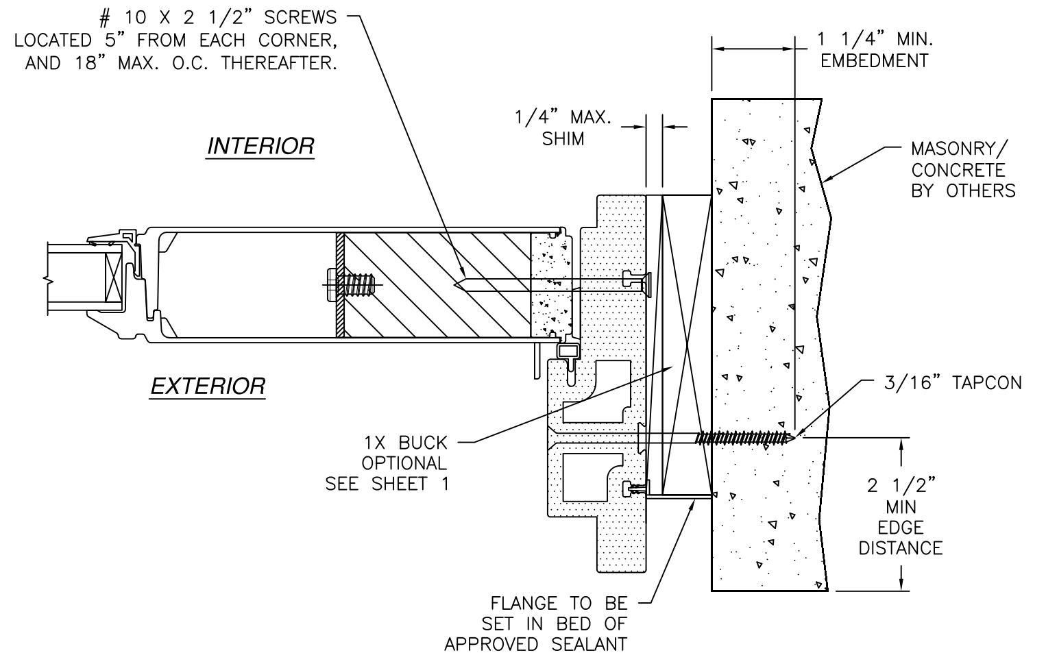
SIDELITE HORIZONTAL CROSS SECTION MASONRY/CONCRETE INSTALLATION
