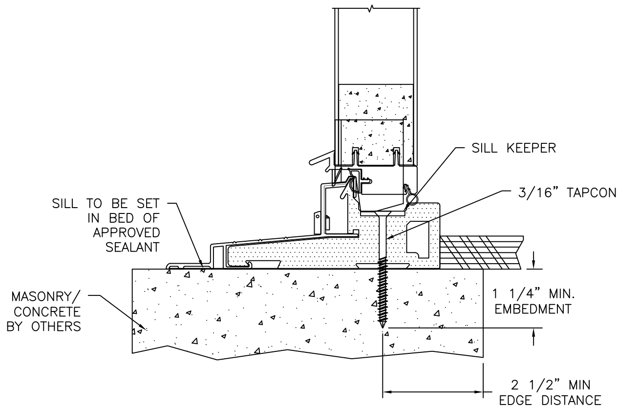
DOOR VERTICAL CROSS SECTION MASONRY/CONCRETE INSTALLATION
