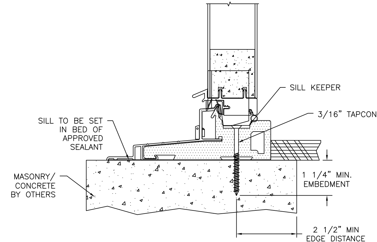
DOOR VERTICAL CROSS SECTION MASONRY/CONCRETE INSTALLATION
