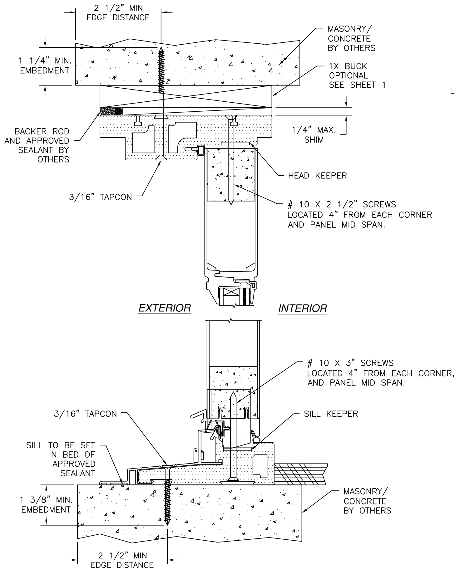
SIDELITE VERTICAL CROSS SECTION MASONRY/CONCRETE INSTALLATION
