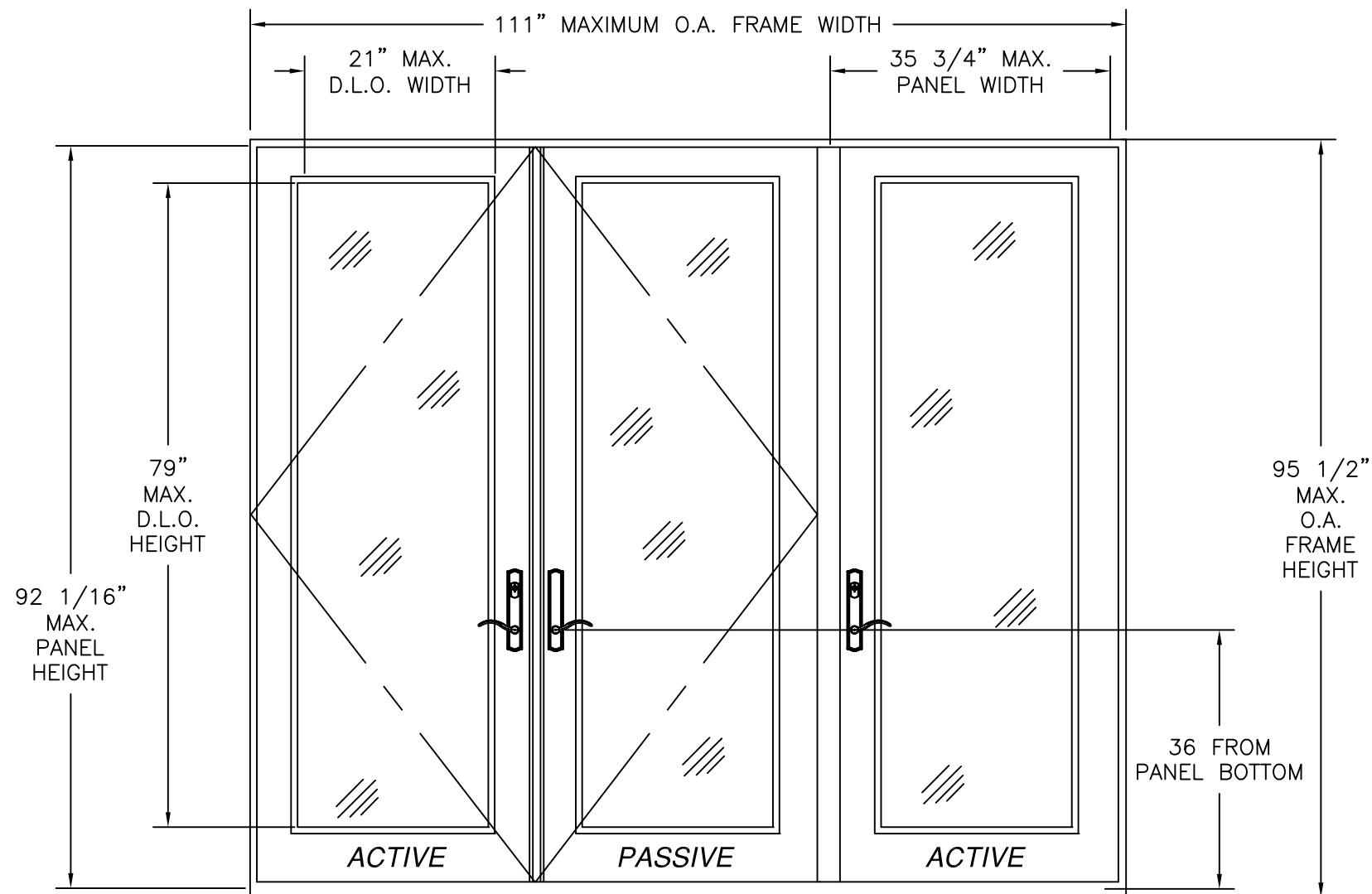
SERIES 9'0 x 8'0 FIBERGLASS IN-SWING GLAZED DOUBLE DOOR W/ SIDELITE EXTERIOR VIEW
