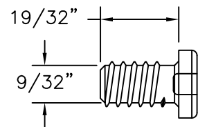
SCREW NYLON 66
