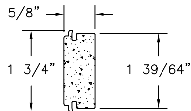
5/8" STILE FOAM PVC
