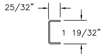
3/32" REINFORCEMENT U-CHANNEL ZINC COATED STEEL .094" THICK
