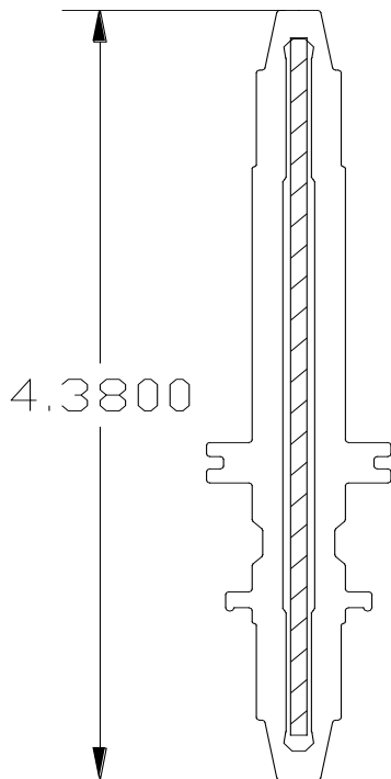
½" Standard Aluminum Mullion w/Stainless Steel Reinforcement Plate Figure 1
