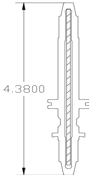
4 ½" Block Frame Mullion End Clip
