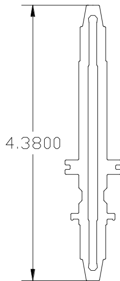
½" Standard Aluminum Mullion
