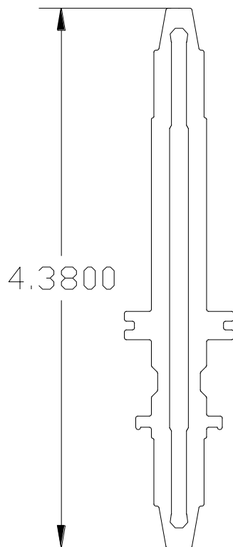
½" Standard Aluminum Mullion Figure 1
