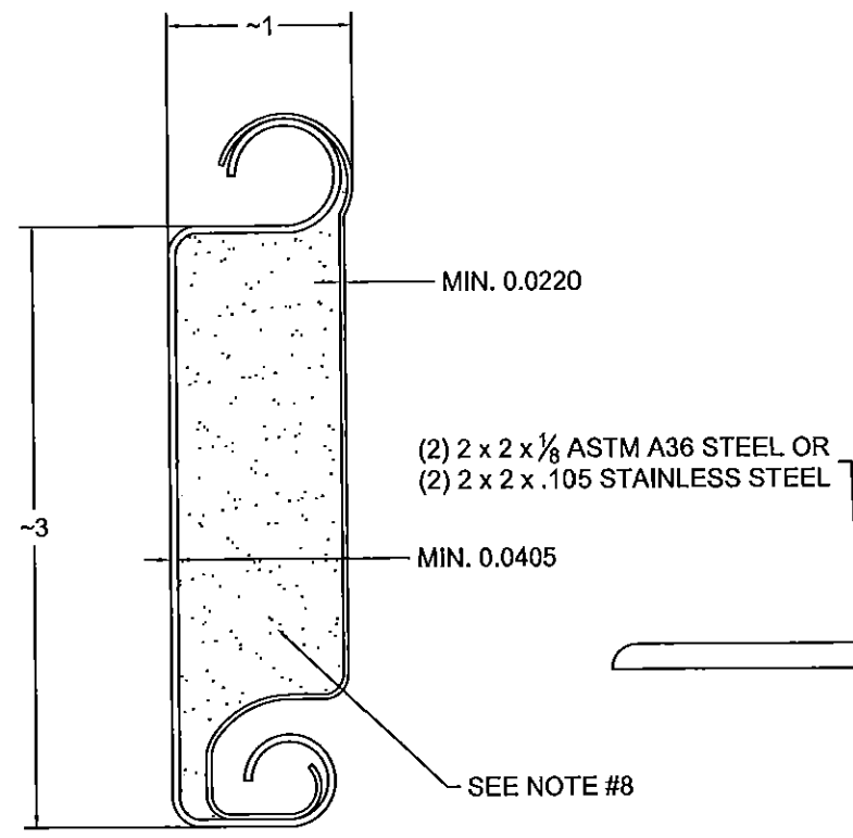
③ SLAT DETAIL TYPICAL SECTION
