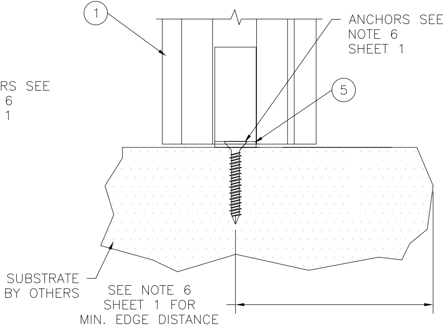
FS-02354 MULLION CLIP INSTALLATION DETAILS SILL, HEAD AND JAMBS TYP. FOR CONCRETE/MASONRY INSTALLATION
