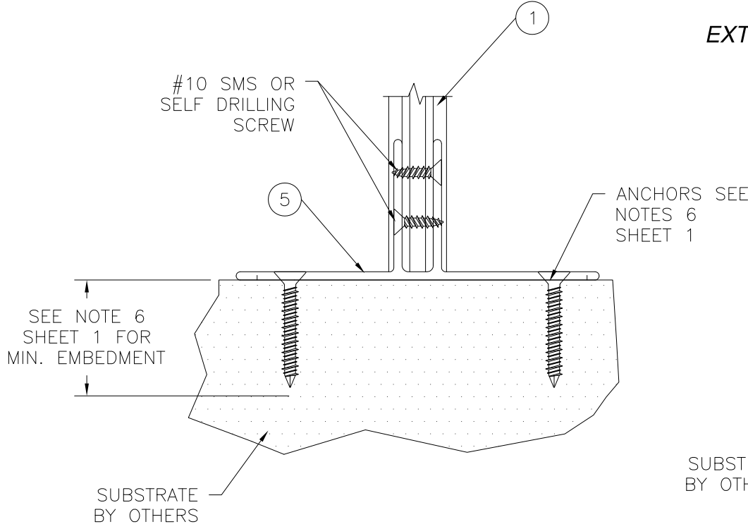
FS-02354 MULLION CLIP INSTALLATION DETAILS SILL, HEAD AND JAMBS TYP. FOR CONCRETE/MASONRY INSTALLATION
