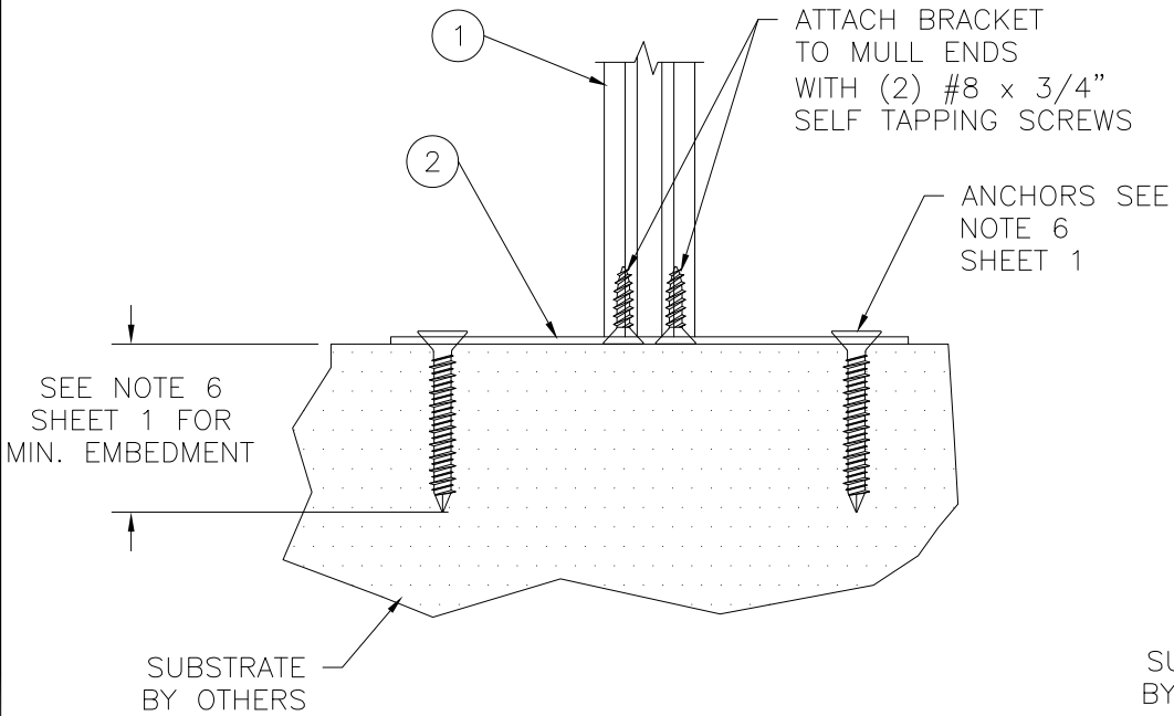
STEEL MULION BRACKET 10203000 INSTALLATION DETAILS SILL, HEAD AND JAMBS TYP. CONCRETE/MASONRY INSTALLATION
