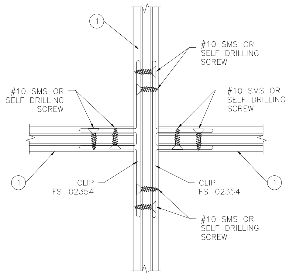
HORIZONTAL TO VERTICAL MULLION CONNECTION
