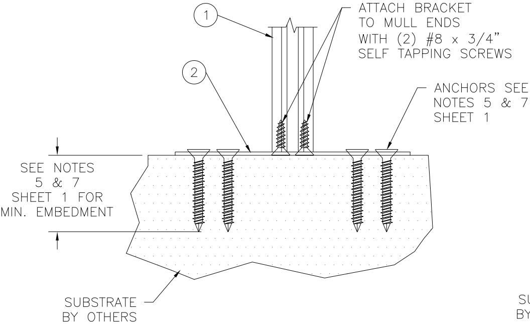
STEEL MULION BRACKET 10203000 INSTALLATION DETAILS SILL, HEAD AND JAMBS TYP. FOR WOOD AND METAL INSTALLATION
