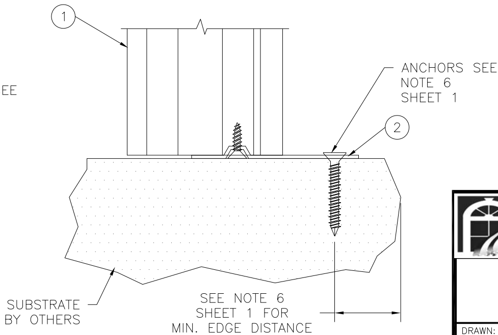
STEEL MULION BRACKET 10203000 INSTALLATION DETAILS SILL, HEAD AND JAMBS TYP. CONCRETE/MASONRY INSTALLATION
