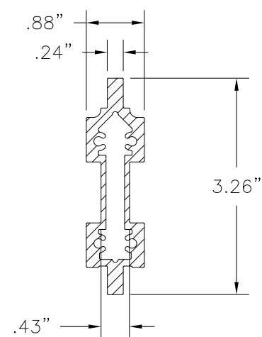
① 10300085 ALUMINUM VERTICAL MULLION ALUMINUM 6005-T5 .075" THICK
