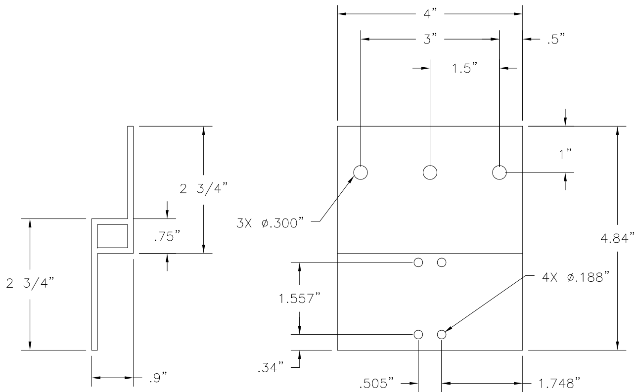
③ MULL CLIP ALUMINUM 6005-T5 .125" THICK
