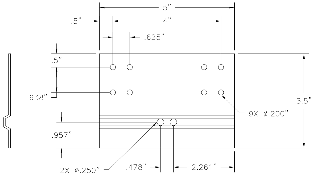
② STEEL MULLION BRACKET 15GA. GALVANIZED STEEL
