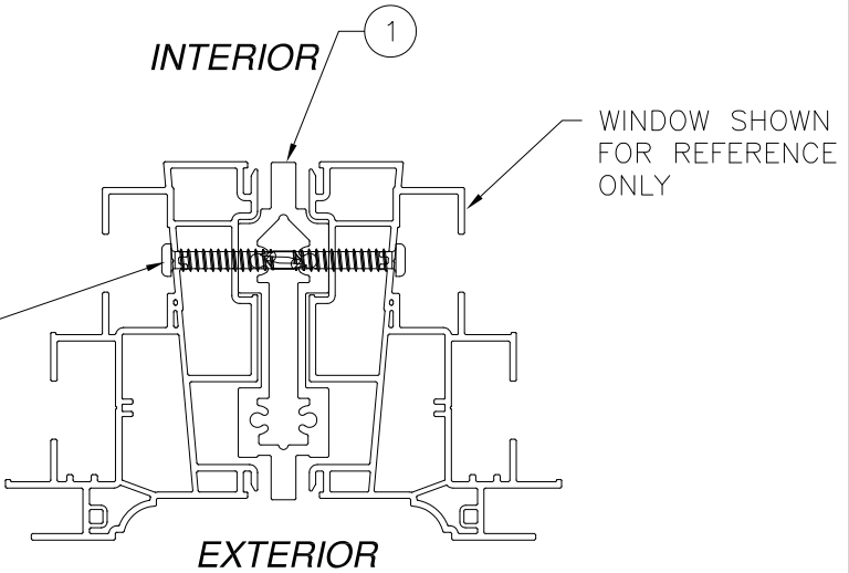
WINDOW TO MULLION INSTALLATION DETAIL
