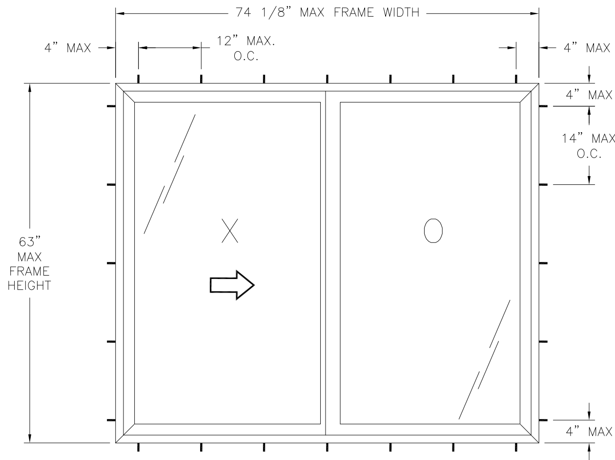
SERIES FWI 1000 ALUMINUM HORIZONTAL SLIDING WINDOW EXTERIOR VIEW FRAME
