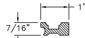
PULL STILE REINFORCEMENT ALUMINUM 6005-T5 (10300207)
