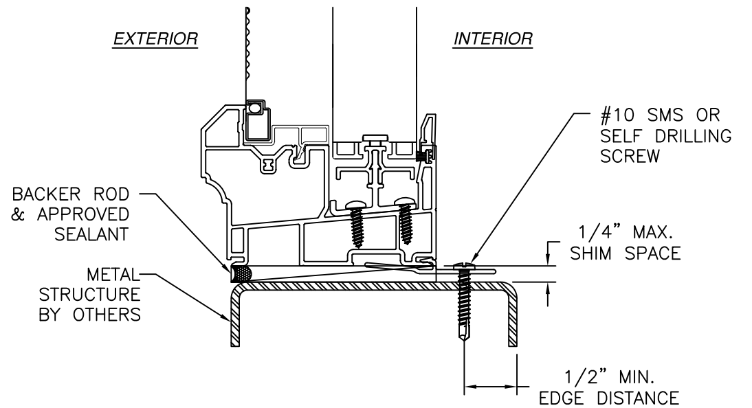
VERTICAL CROSS SECTION METAL STRUCTURE CLIP INSTALLATION
