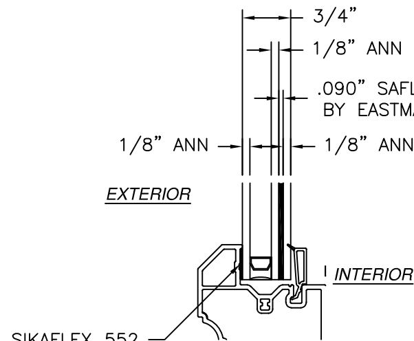
GLAZING DETAIL "C" FIXED GLASS
