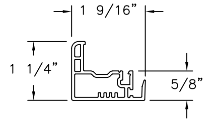
LOCK STILE PVC (10008845)
