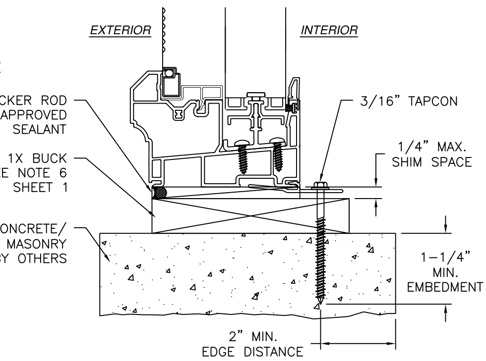
VERTICAL CROSS SECTION CONCRETE/MASONRY 1X BUCK CLIP INSTALLATION FOR INSTALLATION WITHOUT 1X BUCK REFER TO JAMB INSTALLATION DETAIL
