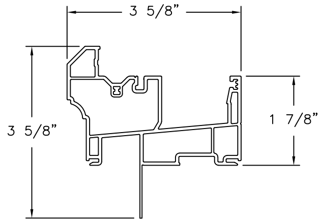
MAIN FRAME FIN INSTALLATION PVC (10008684)
