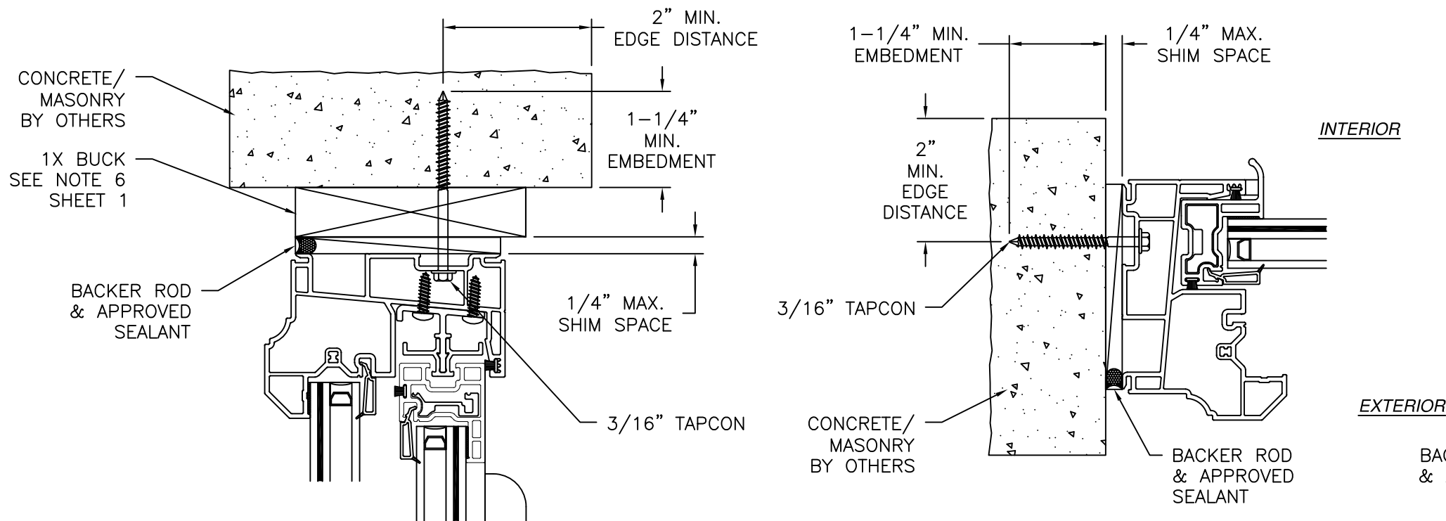
JAMB INSTALLATION DETAIL CONCRETE/MASONRY INSTALLATION FOR 1X BUCK INSTALLATION REFER TO HEAD AND SILL INSTALLATION DETAILS
