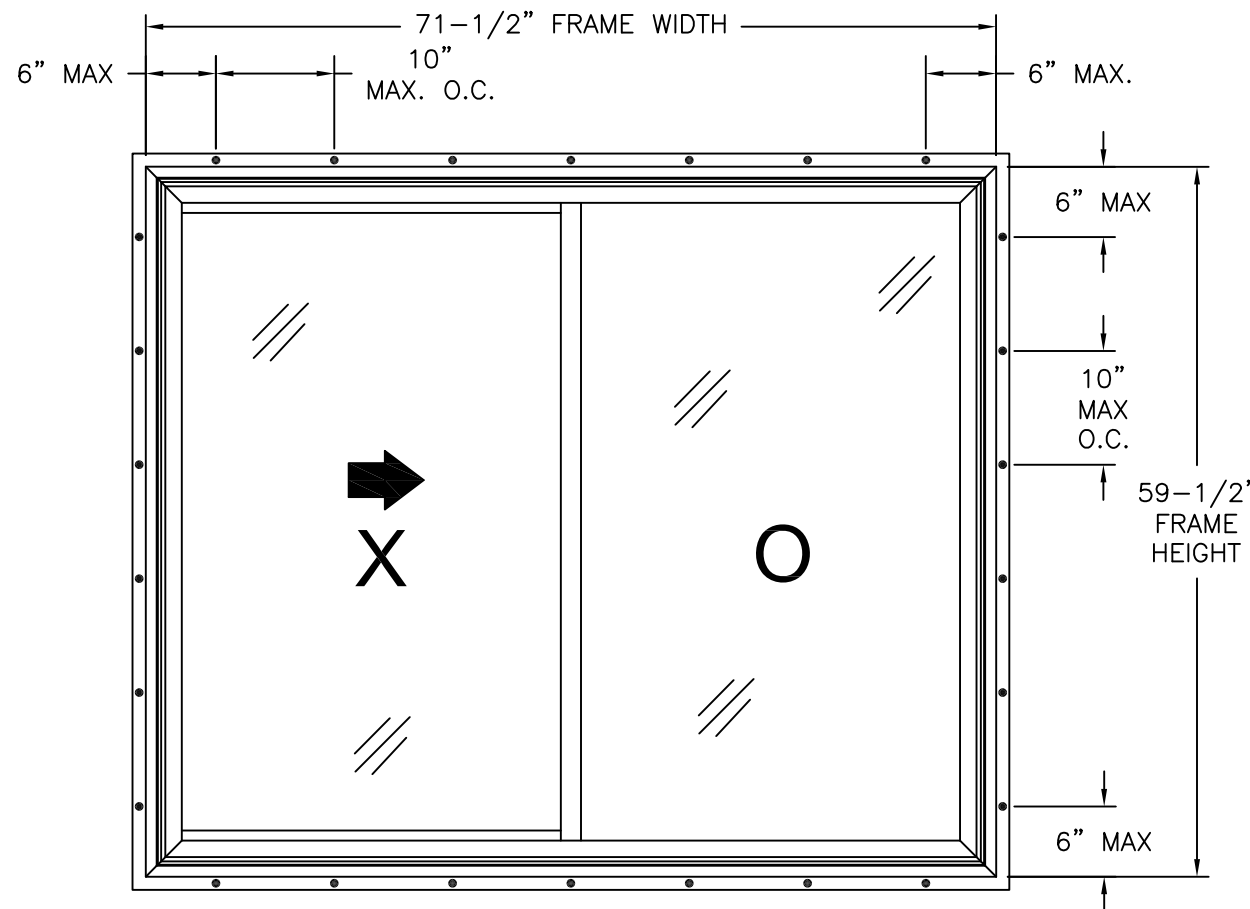
SERIES 4241 HORIZONTAL SLIDING WINDOW
