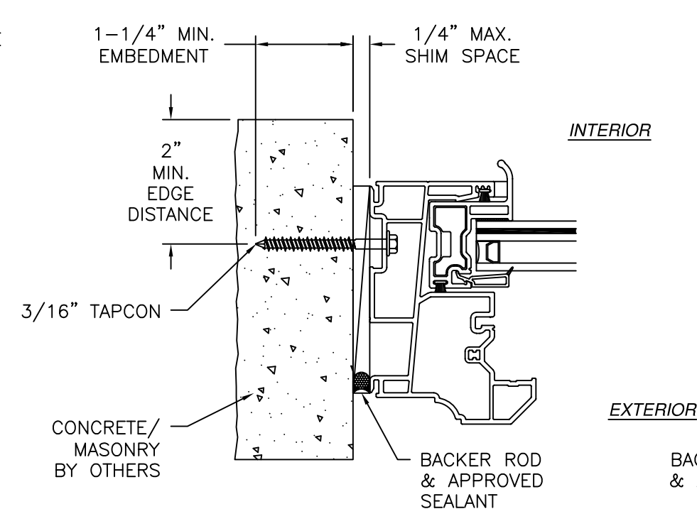
JAMB INSTALLATION DETAIL CONCRETE/MASONRY INSTALLATION FOR 1X BUCK INSTALLATION REFER TO HEAD AND SILL INSTALLATION DETAILS
