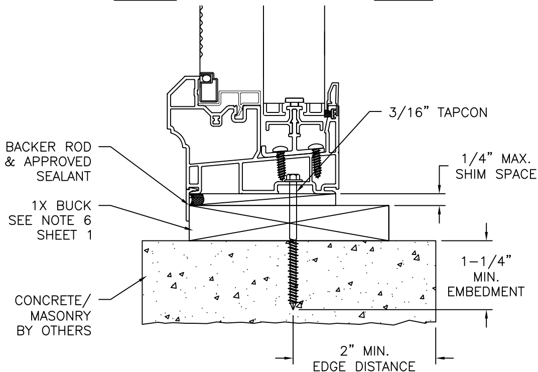
VERTICAL CROSS SECTION CONCRETE/MASONRY 1X BUCK INSTALLATION FOR INSTALLATION WITHOUT 1X BUCK REFER TO JAMB INSTALLATION DETAIL
