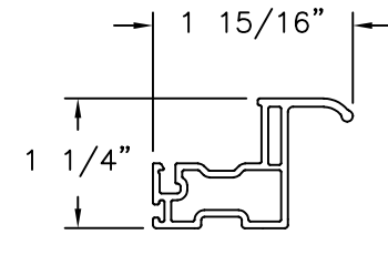
PULL STILE PVC (10008882)
