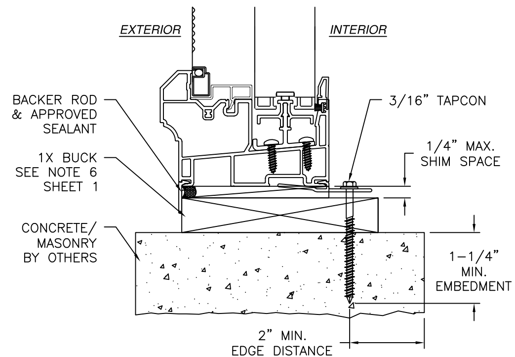
VERTICAL CROSS SECTION CONCRETE/MASONRY 1X BUCK CLIP INSTALLATION FOR INSTALLATION WITHOUT 1X BUCK REFER TO JAMB INSTALLATION DETAIL
