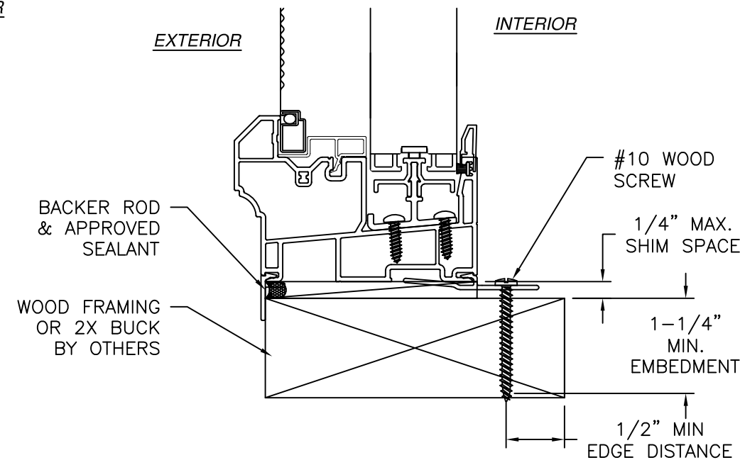
VERTICAL CROSS SECTION WOOD FRAMING OR 2X BUCK CLIP INSTALLATION
