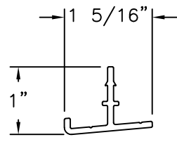
SLIDER TRACK ALUMINUM 6005-T5 (10300189)
