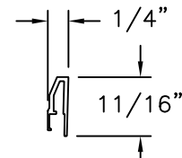
SILL EXTENDER PVC (20008052)
