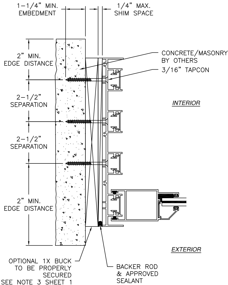
JAMB INSTALLATION DETAIL CONCRETE/MASONRY INSTALLATION
