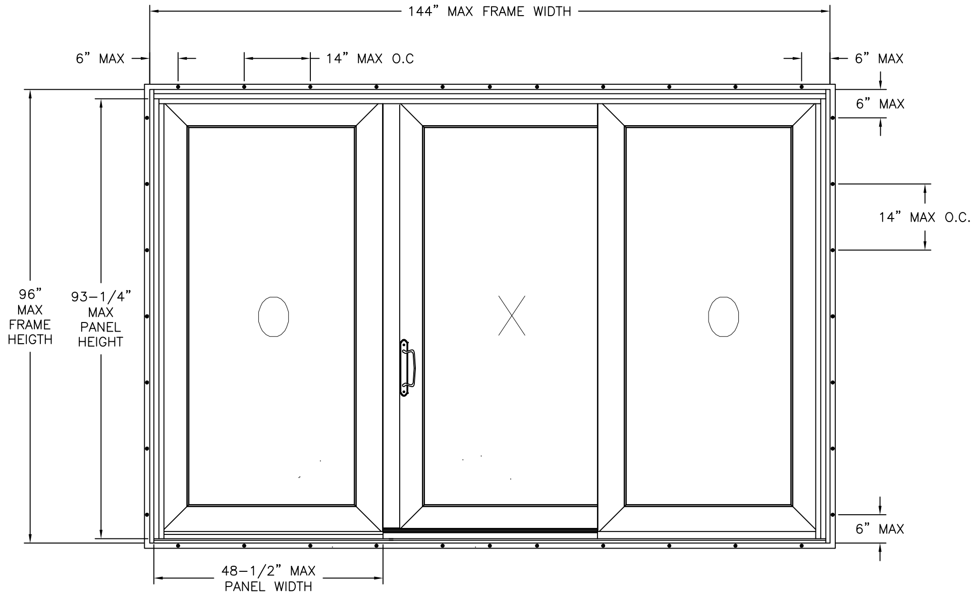
SERIES 623 VINYL SGD EXTERIOR VIEW FIN INSTALLATION
