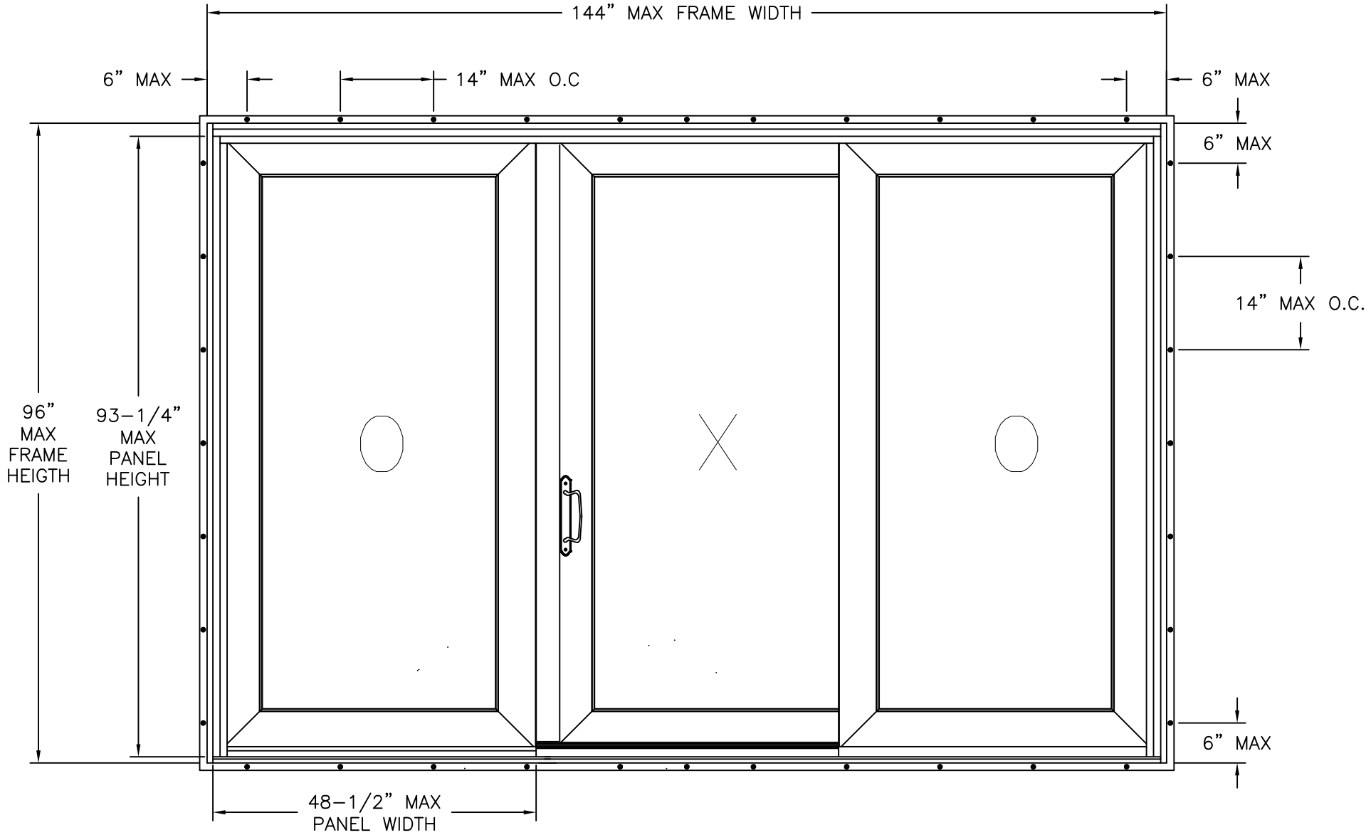
SERIES 623 VINYL SGD EXTERIOR VIEW FIN INSTALLATION
